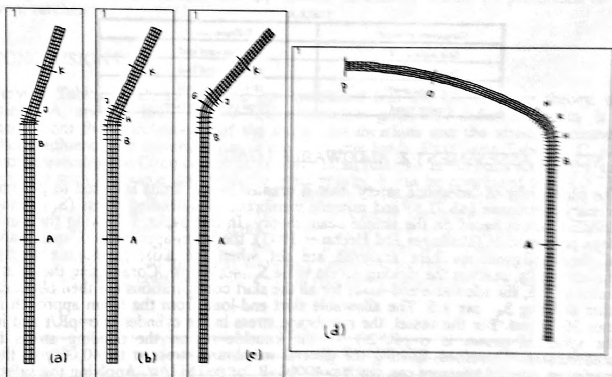
Figure-1 - (a) Skirt with \alpha=18^\circ , (b) Skirt with \alpha=25^\circ , (c) Skirt with \alpha=45^\circ , and (d) Pressure Vessel
