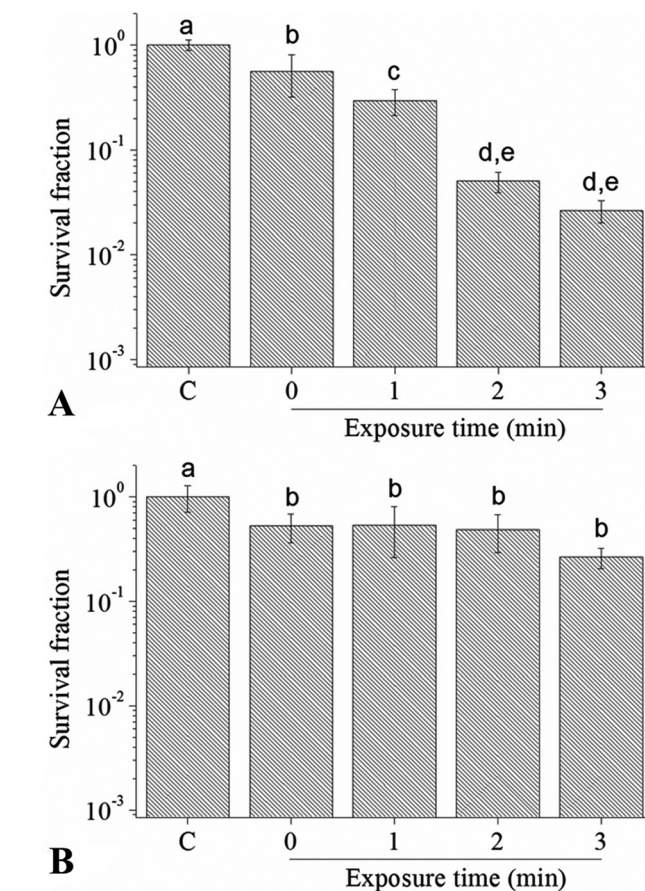
Fig. 1 Effect of MB ( 30\ \mu\text{M} ) on the photoinactivation of E. coli in (A) water and (B) saline solution. Irradiation was performed with a 660 nm laser, power of 40 mW and irradiance of about 100\ \text{mW cm}^{-2} . Different letters mean statistically significant differences.
