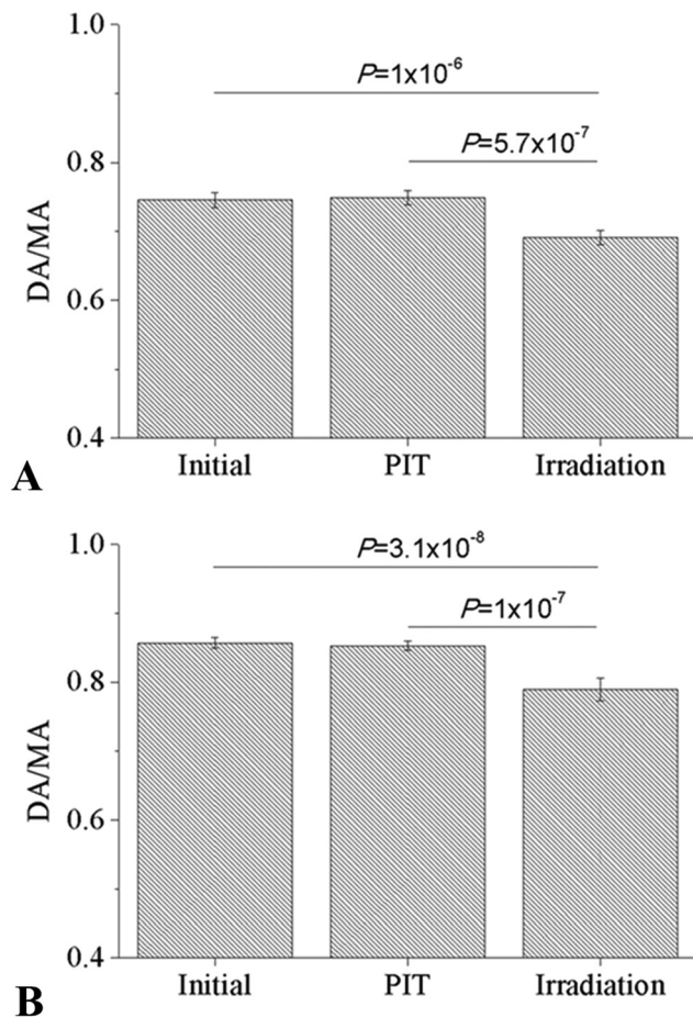
Fig. 4 DA/MA (dimer absorbance/monomer absorbance ratio) for MB (30 μM) in (A) water and (B) saline solution. Pre-irradiation time (PIT) represents measurements conducted 3 min after incubation of bacterial suspension with MB.
