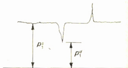
Fig. 2. Scheme of a multiple reflection pattern. The intensities, p_1^s due to a single reflection, and p_1^d due to a double reflection, are recorded at the same scale.
