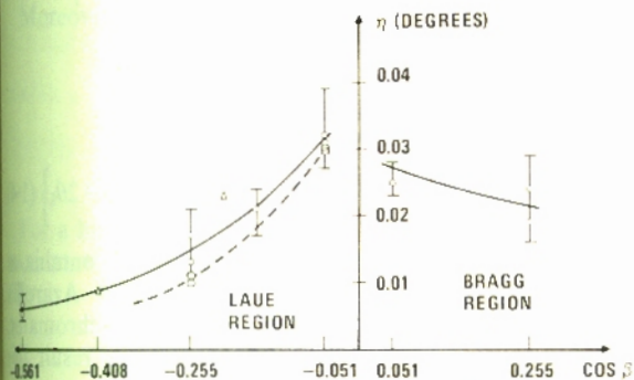
Fig. 4. Germanium plate. Some results from preliminary measurements made with Mo K\alpha . \circ Primary reflection: 111; values calculated without polarization correction for secondary reflecting planes diffracting in a direction forming an angle \beta with the normal to the plate. \square Values for the same secondary reflecting planes taking polarization into account. \triangle Primary reflection: 222. Each point was obtained from a pair of planes diffracting in directions which form the same angle with the normal. The bars across the experimental points indicate the uncertainty arising from the estimated error in the measured value of R .
