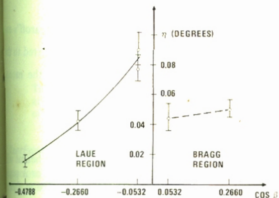
Fig. 5. Silicon plate. Some results from preliminary measurements made with Mo K\alpha . Primary reflection: 111. The branch of the curve in the Bragg region has the wrong slope; this is probably due to experimental error.
