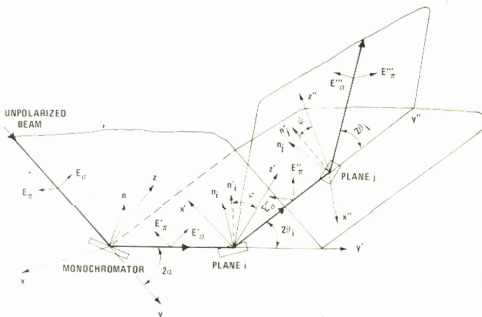
Fig. 3. Illustrating the nomenclature used in the calculation of polarization factors. E_\sigma indicates the electric field component in the plane of incidence and E_\pi the component normal to it. The Z axis is in the plane of incidence and normal to the incident beam, n'_i is the projection of the normal n_i to the plane i onto the x'z' plane. The angle \varphi depends on the experimental set up, while \psi can be expressed as a function of 2\theta_i , 2\theta_j and 2\theta_k .
