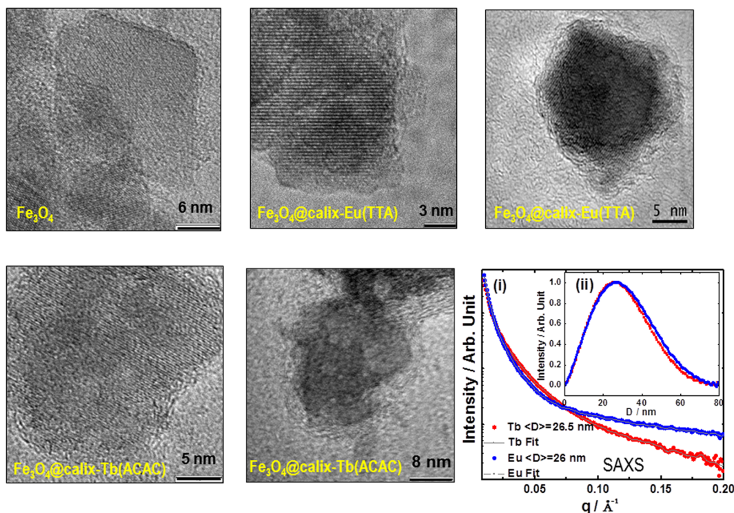
Figure 3. High-resolution TEM images of (clockwise from top left): \text{Fe}_3\text{O}_4 , \text{Fe}_3\text{O}_4@ \text{calix-Eu(TTA)} nanoparticles (different magnifications), \text{Fe}_3\text{O}_4@ \text{calix-Tb(ACAC)} one (different magnifications). SAXS profile of \text{Fe}_3\text{O}_4@ \text{calix-Eu(TTA)} and \text{Fe}_3\text{O}_4@ \text{calix-Tb(ACAC)} shows (i) scattering intensity as a function of the scattering vector and (ii) the size distributions obtained from the fit on SAXS data for the \text{Fe}_3\text{O}_4@ \text{calix-Eu(TTA)} and \text{Fe}_3\text{O}_4@ \text{calix-Tb(ACAC)} .
