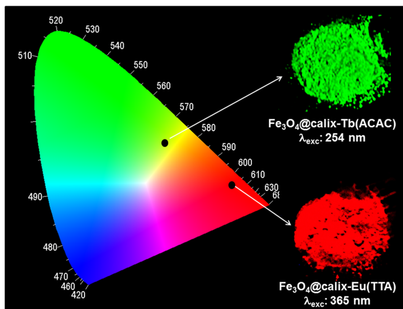
Figure 8. CIE chromaticity diagram showing the (x, y) emission color coordinates for \text{Fe}_3\text{O}_4@ \text{calix-Eu(TTA)} and \text{Fe}_3\text{O}_4@ \text{calix-Tb(ACAC)} nanophosphors irradiated at different wavelengths. Photographs of nanomaterials (inset) taken with a digital camera displaying the green and red emissions under UV irradiation lamp at 254 and 365 nm, respectively.
