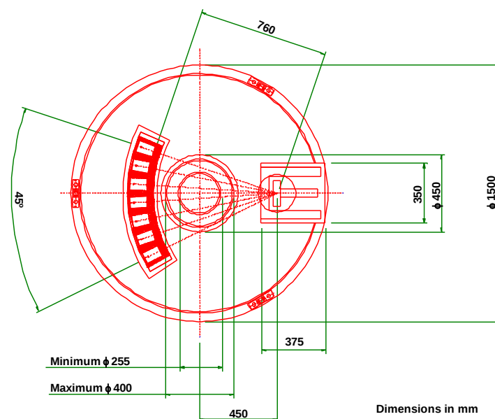
Figure 1. Top view drawing of the CT used.
