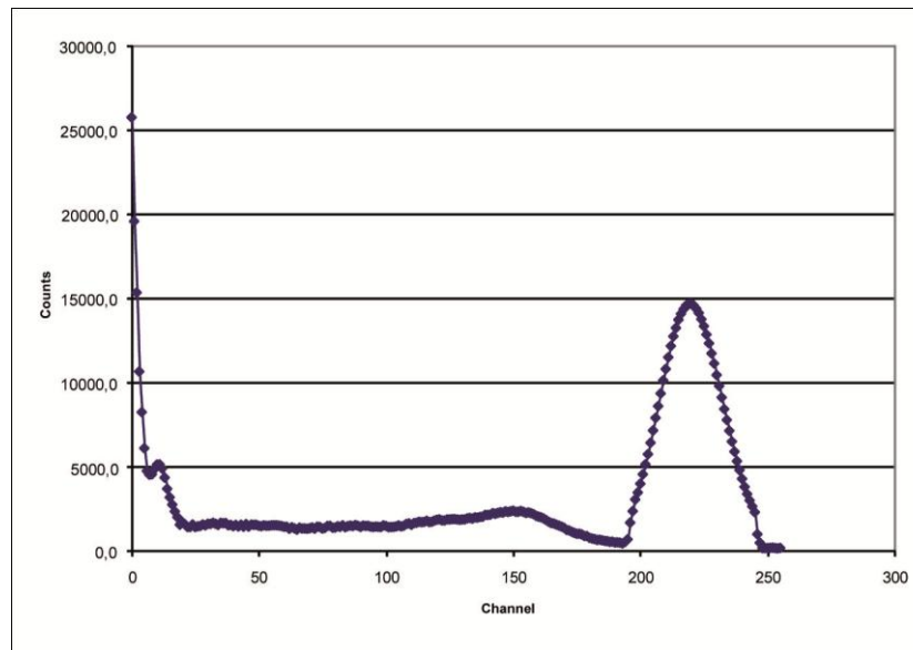
Figure 2. Energy spectrum of the (667 keV) ^{137}\text{Cs} gamma radiation.
