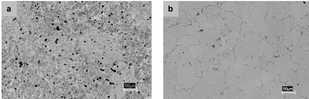
Fig. 2 - SEM micrographs of the powder metallurgic processed Ti-based alloys. a) Ti-13Nb-13Zr alloy - general aspect, note the residual pores and (b) Ti-35Nb-7Zr-5Ta alloy showing a good densification, with complete dissolution of alloying elements in the titanium matrix.
