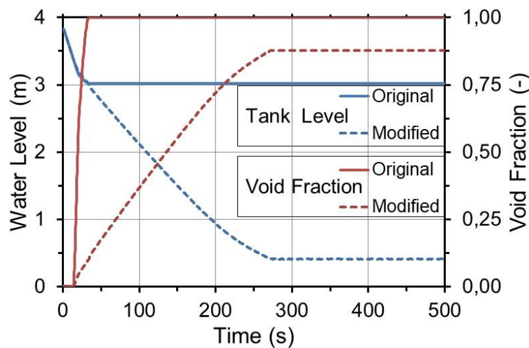
Figure 4 - Comparison of water tank level and siphon breaker line entrance void fraction for original RELAP5/RMB against a modified version inducing siphon breaker failure.
