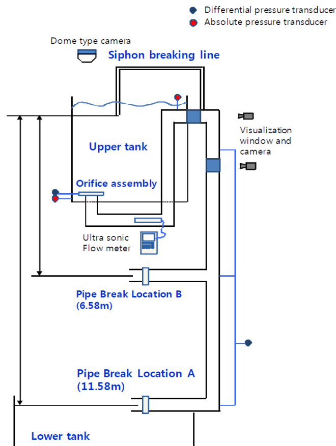
Figure 1 - Schematic representation of POSTECH siphon breaker test facility.
