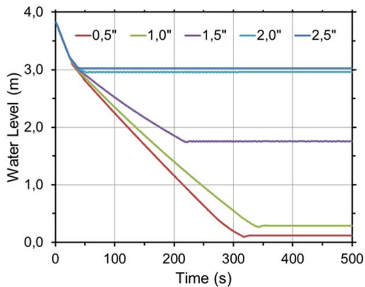
Figure 6 - RELAP5/RMB results for several siphon breakers line diameters for LOCA at intermediate position.
