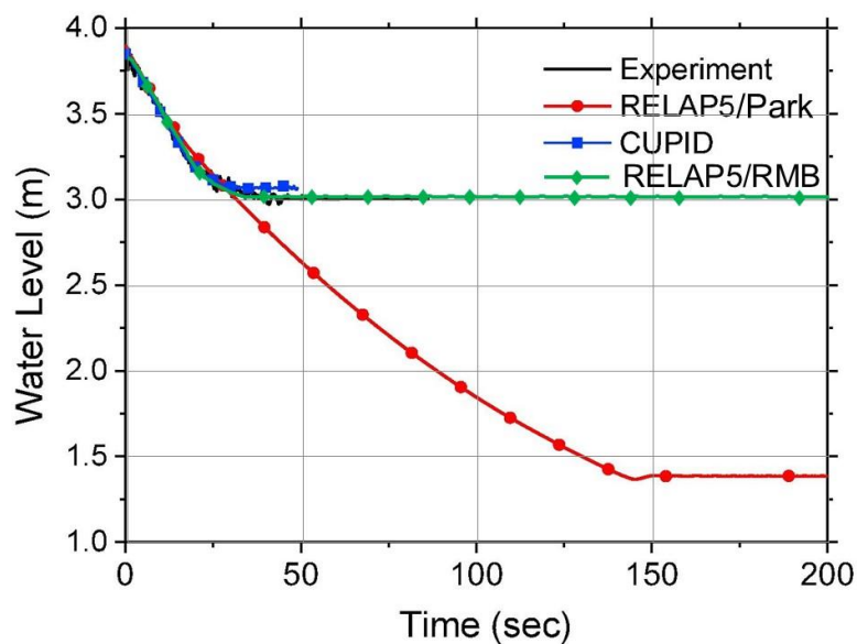
Figure 3 - Comparison of RELAP5/RMB results against POSTECH experimental and numerical
