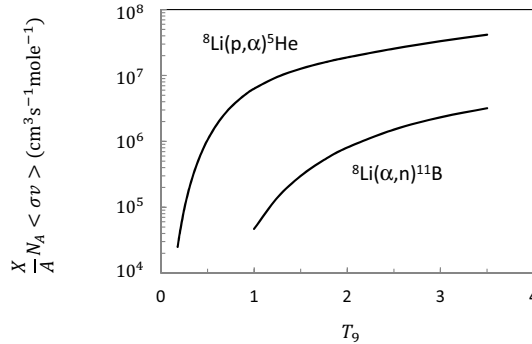
Figure 2. The {}^8\text{Li}(p,\alpha){}^5\text{He} and {}^8\text{Li}(\alpha,n){}^{11}\text{B} reaction rates multiplied by the proton and \alpha mass fractions.
