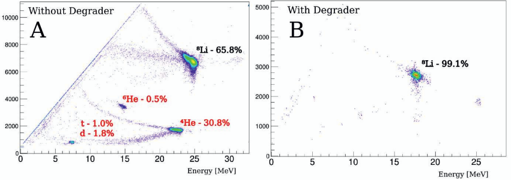
Figure 3. Bidimensional energy spectra obtained using a Si telescope at \Theta_{\text{lab}}=10^\circ , in the large chamber after the second solenoid, with the secondary beams focused on a gold target. Spectrum A was obtained without a degrader and spectrum B with a degrader.
