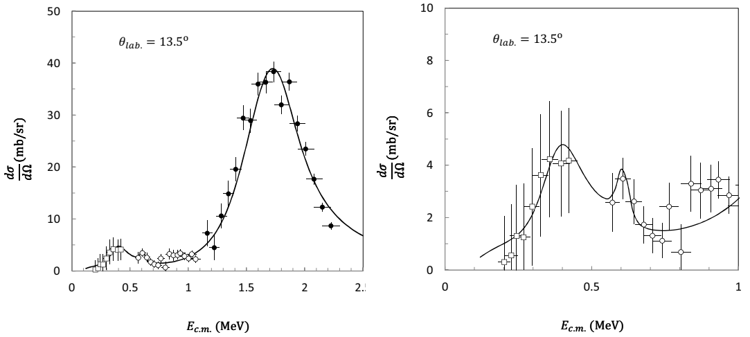
Figure 1. The spectrum on the left shows the {}^8\text{Li}(p,\alpha){}^5\text{He} differential cross sections at \theta_{\text{lab}} = 13.5^\circ , with the R -matrix fit (solid line.) In the spectrum on the right we present the same reaction, performing a zoom on the low energy resonances and their R -matrix-fit.
