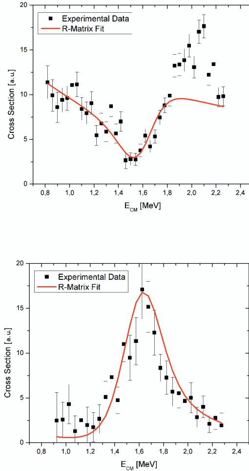
Figure 5. The excitation function of the ^8\text{Li}(p,p)^8\text{Li} reaction, together with a fit by the R-matrix calculation is shown on the top. On the bottom is the excitation function of the ^8\text{Li}(p,\alpha)^5\text{He} reaction, together with a fit by the R-matrix calculation.
