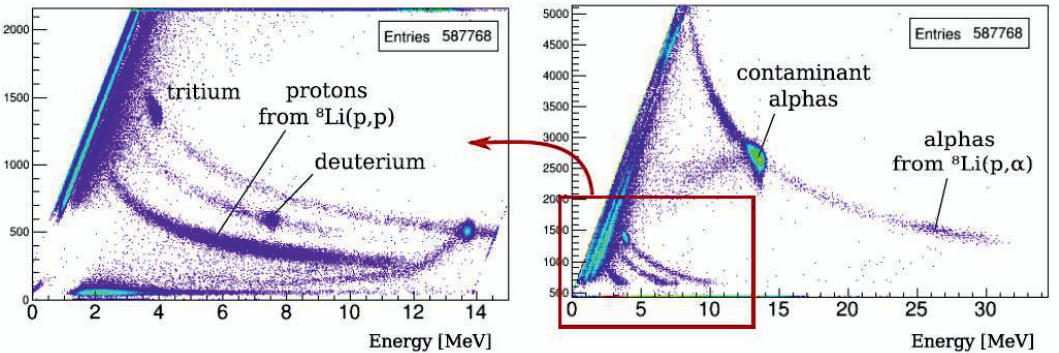
Figure 4. Bidimensional energy spectra obtained using a Si telescope at \Theta_{\text{lab}}=10^\circ , in the large chamber after the second solenoid, with the secondary beams focused on a [\text{CH}_2]_n target. The spectrum on the left is a zoom of the spectrum on the right.
