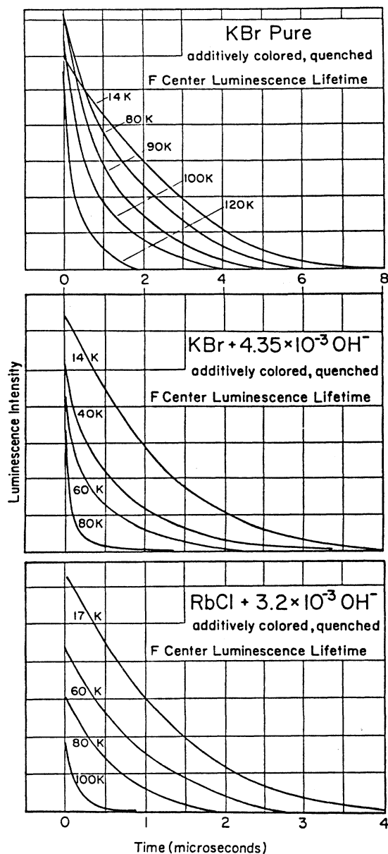
FIG. 3. The time dependence of the F luminescence signal excited by a pulsed laser of 10 nsec of time duration and tuned at the main F absorption band in pure and \text{OH}^- doped KBr and RbCl crystals at several temperatures for the nonaggregated case.
