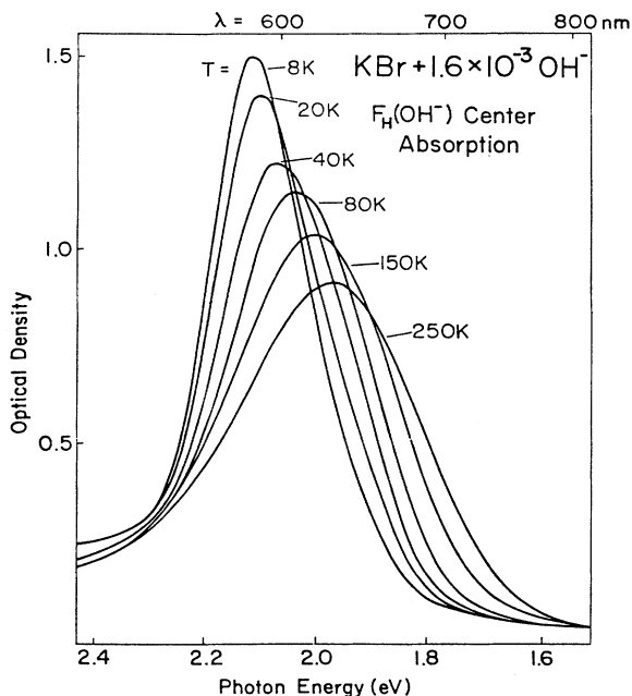
FIG. 6. Spectral dependence of F_H(\text{OH}^-) absorption band in \text{KBr} at several temperatures.
