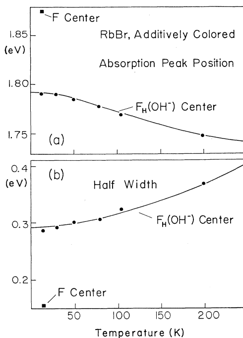
FIG. 5. Temperature dependence of peak position (a) and half width (b) of F_H(\text{OH}^-) absorption in RbBr.
