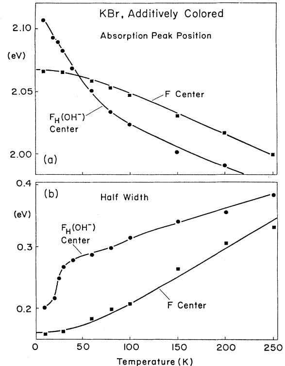
FIG. 7. Temperature dependence of peak position (a) and half width (b) of F_H(\text{OH}^-) absorption in \text{KBr} .
