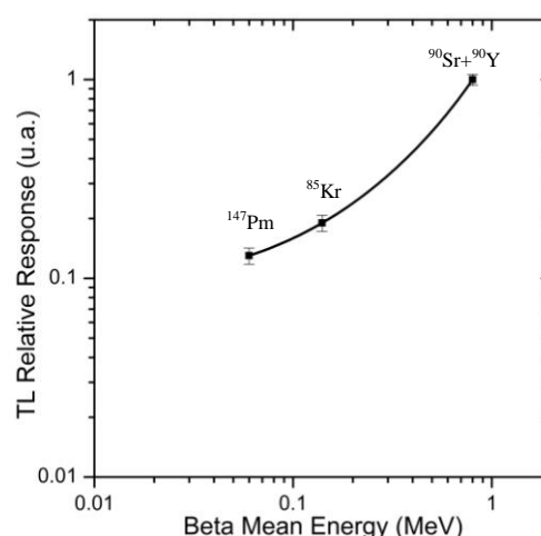
Fig 5. Energy dependence of the detectors exposed to beta radiation sources (BSS2 system).
