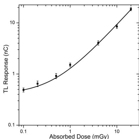
Fig. 4. TL dose-response curve of the detectors exposed to ^{90}\text{Sr}+^{90}\text{Y} system.
