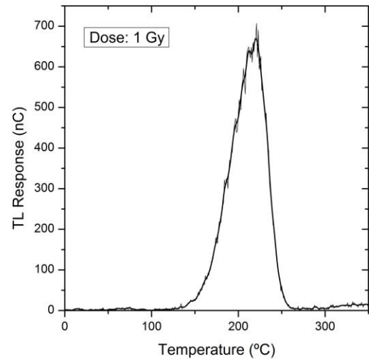
Fig. 3. TL glow curve of a BeO pellet irradiated with 1 Gy of ^{90}\text{Sr}+^{90}\text{Y} (BSS1).
