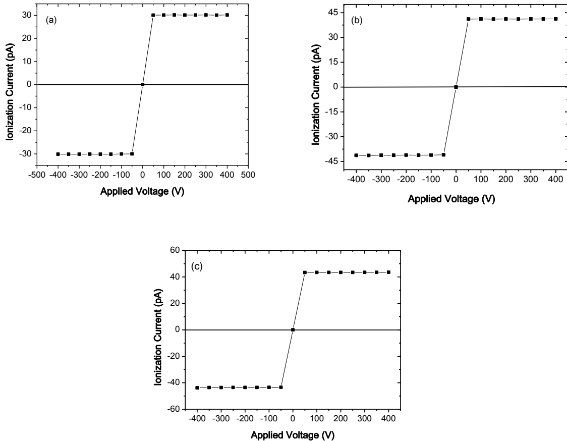
Figure 1: Saturation curves of the ionization chambers for the radiation quality RQT 9: (a) C1; (b) C2; (c) C3. The maximum measurement uncertainty was 0.59%.
