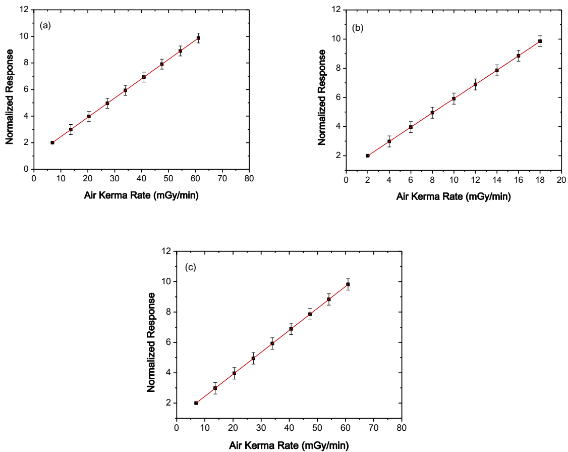
Figure 2: Linearity of response to quality RQT 9 of the ionization chambers: (a) C1; (b) C2; (c) C3. The linear correlation coefficient in all cases is R^2=1.000 .
