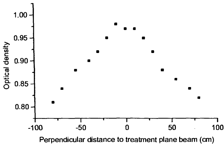
Figure 3b. Field flatness in the treatment vertical plane.
