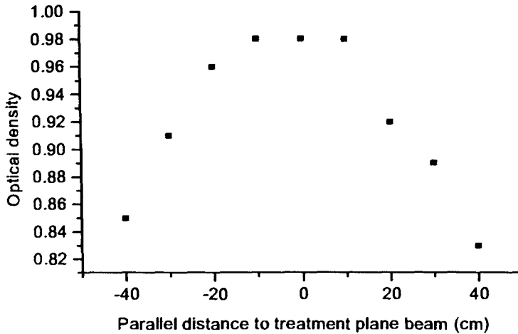
Figure 3a. Field flatness in the treatment horizontal plane.
