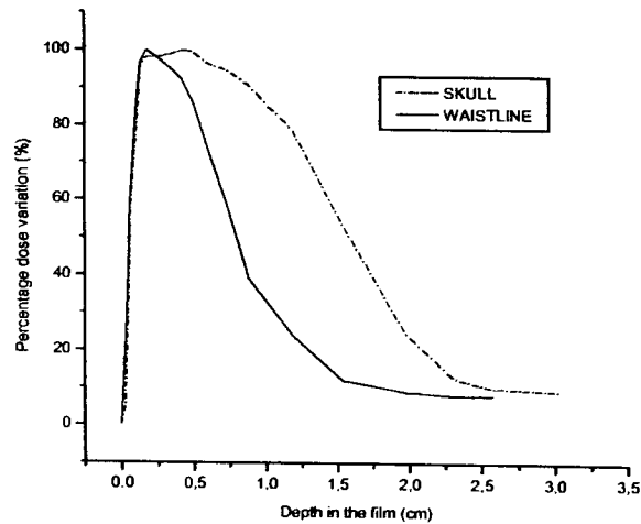
Figure 6. Relative depth dose presented by the dosimetric films placed into the antropomorphic phantom.
