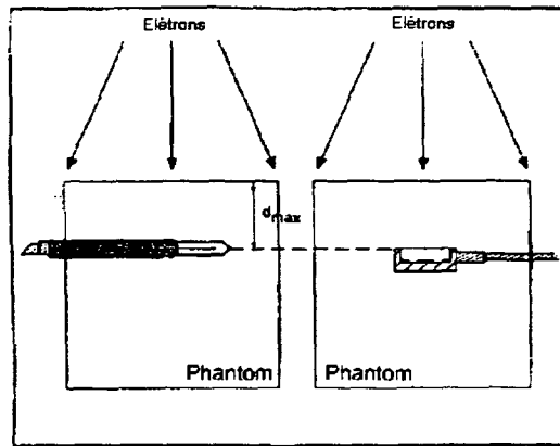
Figure 4. Geometry used to calibrate the parallel-plate chamber (right) with the Farmer chamber (left).
