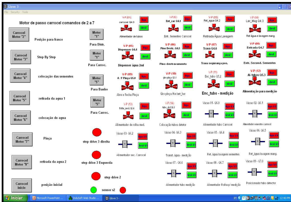
FIG 3 - InduSoft Web Studio 6.1 supervisory – computer control.
