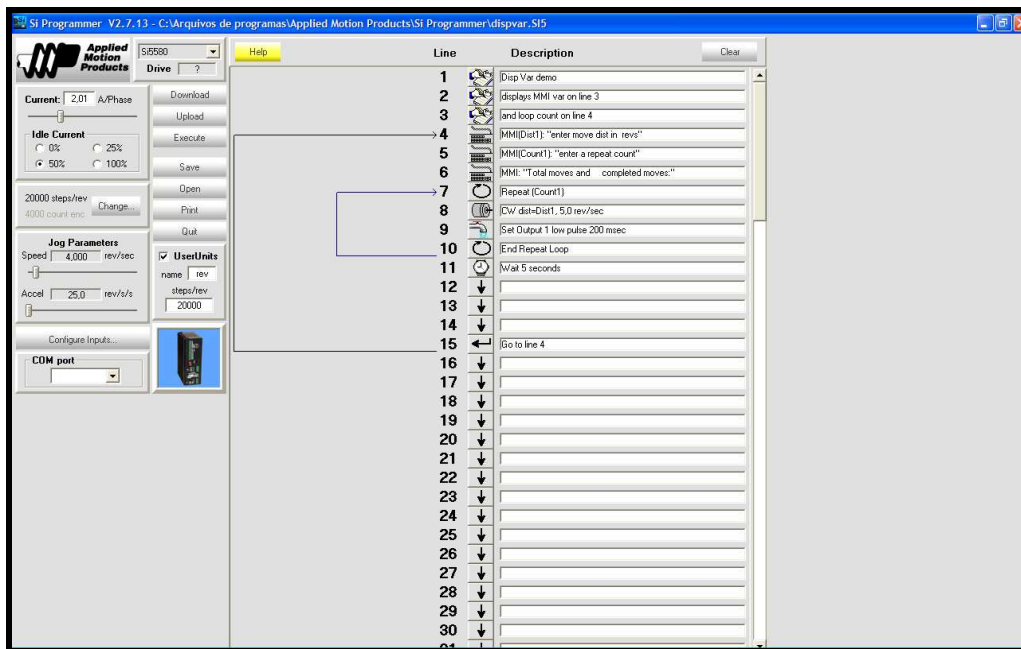
FIG 6- Applied Motion drives of the stepper motors.
