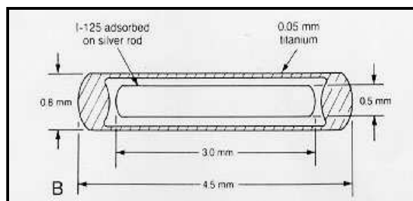
FIG 1. Iodine-125 radioactive seed produced at IPEN – CNEN/SP.
