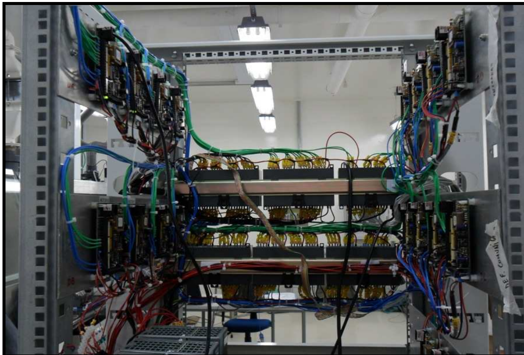
FIG 5 - Siemens Programmable Logic Controller (PLC) and Step motors driver.
