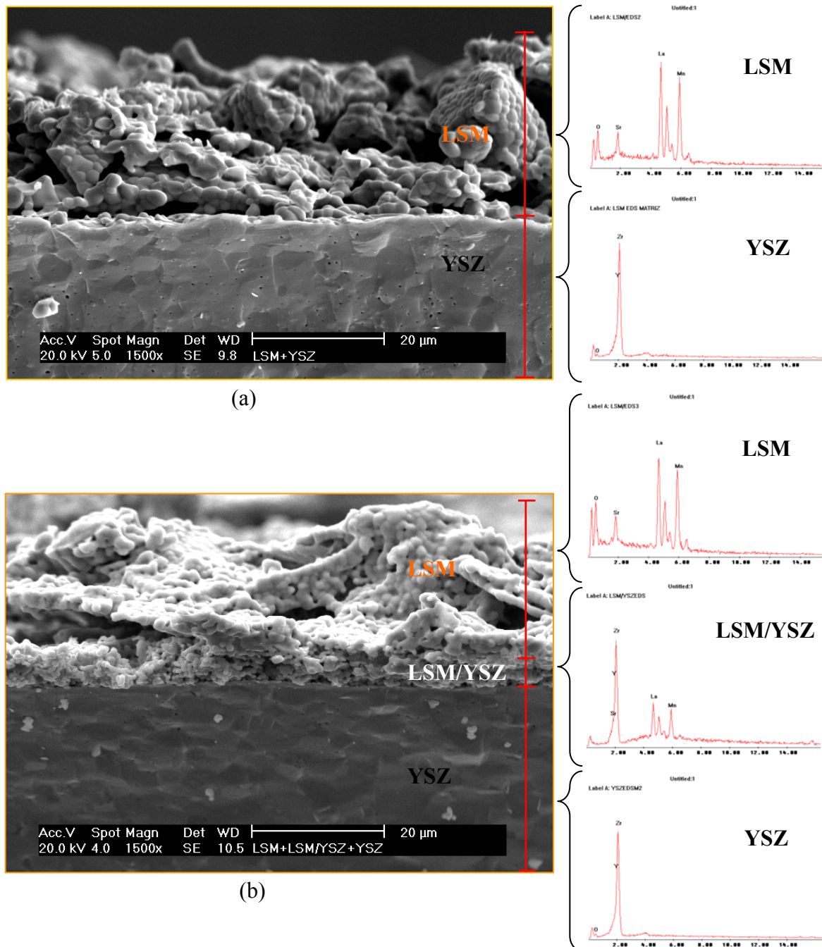
Figure 3 - Micrographs of the transversal sections of the LSM (a) and LSM + LSM/YSZ (b) thin films on YSZ substrate obtained by SEM and energy spectra of each film and substrate obtained by EDS.
