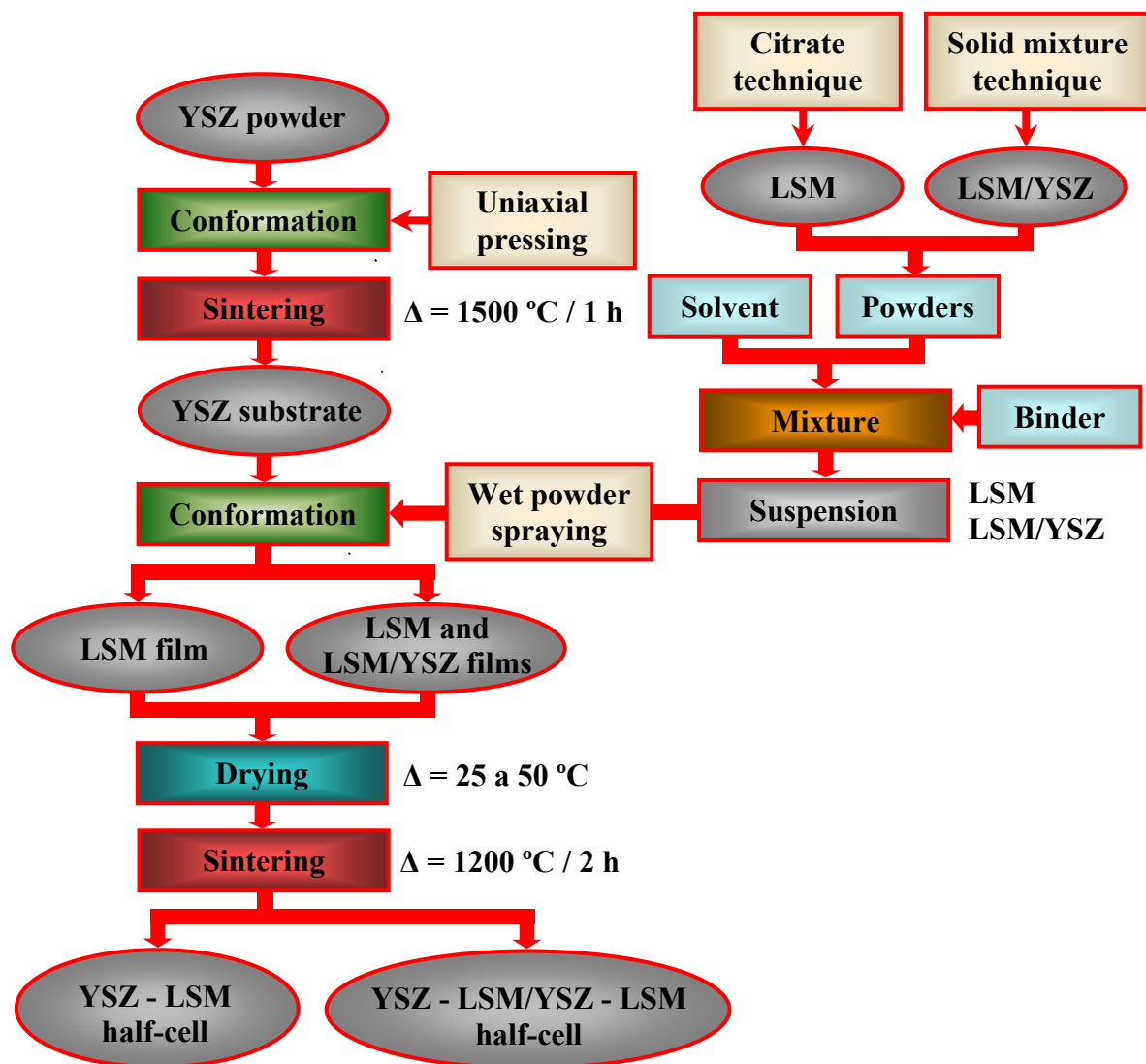
Figure 1 - Ceramic processing for the conformation of the half-cells.
