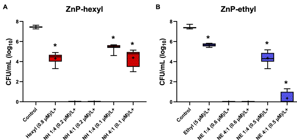
Figure 6 Box plots of photoinactivation of C. albicans yeasts. The photoefficiency was evaluated with individual ZnPs (A) ZnP-hexyl at 0.8 \text{ }\mu\text{M} and (B) ZnP-ethyl at 5.0 \text{ }\mu\text{M} or in association with AgNPs (1:4 and 4:1 v/v ratio) at different PS concentrations. ZnP concentrations are given in parenthesis. The pre-irradiation incubation time was 10 min and the light dose was 4.3 \text{ J/cm}^2 . Hexyl: ZnP-hexyl; Ethyl: ZnP-ethyl; NH: AgNPs-ZnP-hexyl; NE: AgNPs-ZnP-ethyl. L+: with irradiation. At least three independent experiments were performed in triplicate; * p < 0.05 in relation to the control.
