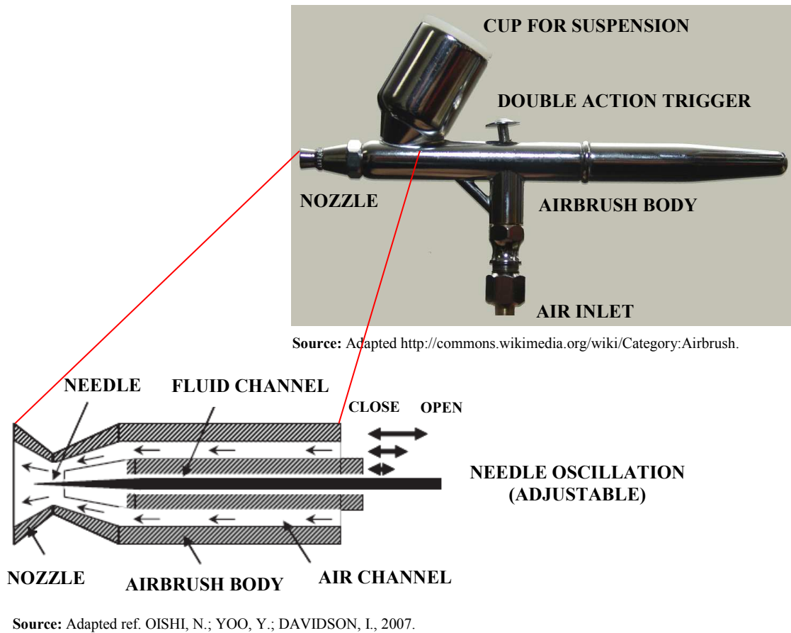
Fig. 1 - Equipment airbrush and cross section diagram.
