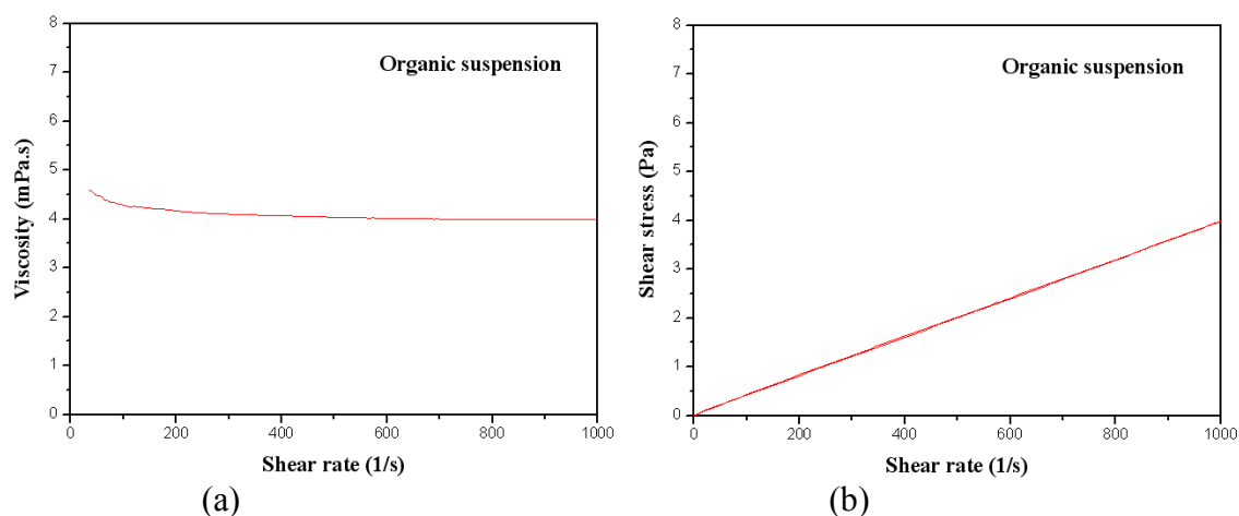
Fig. 3 – Flow (a) and viscosity (b) curves of the LSM organic suspension.
