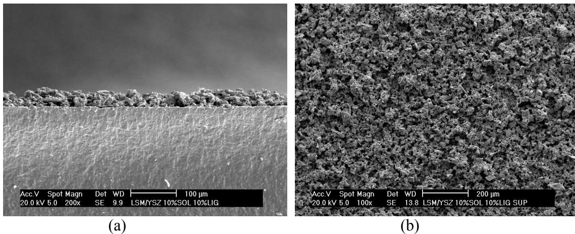
Fig. 5 - Micrographs of the cross section of the LSM ceramic film on the YSZ electrolyte substrate (a) and cathodic ceramic film surface (b).
