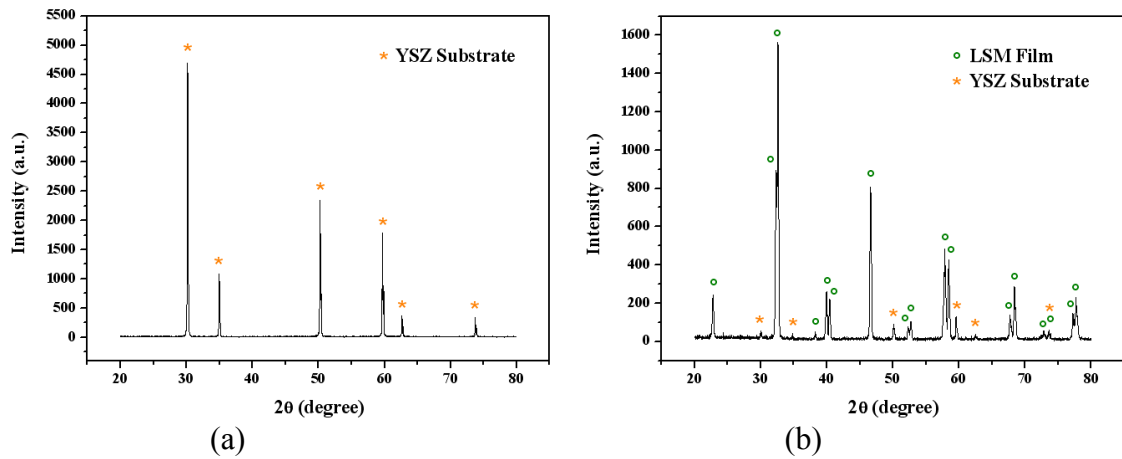
Fig. 4 - Diffractograms of the YSZ electrolyte substrate (a) and of the LSM ceramic film (b).
