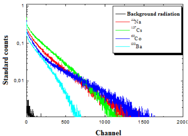
Figure 9: Spectra obtained for the radiation of ^{137}\text{Cs} , ^{60}\text{Co} , ^{22}\text{Na} e ^{133}\text{Ba} sources with CsI:Pb 10^{-2} M crystal.
