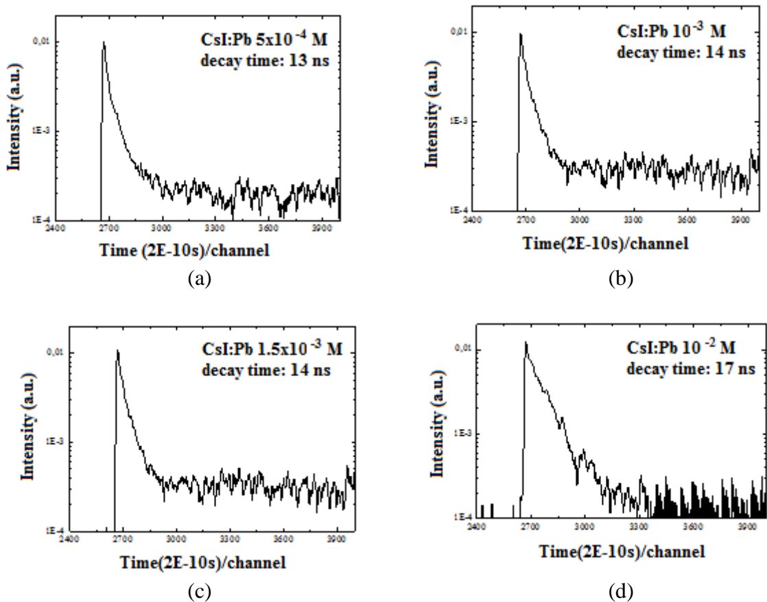
Figure 5: Luminescence decay time spectra of CsI: Pb crystals at various concentrations: (a) 5 \times 10^{-4} M, (b) 10^{-3} M, (c) 1,5 \times 10^{-3} M and (d) 10^{-2} M.
