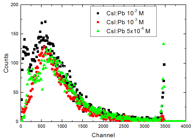
Figure 10: Results of the measurements using CsI:Pb crystal and neutron source.
