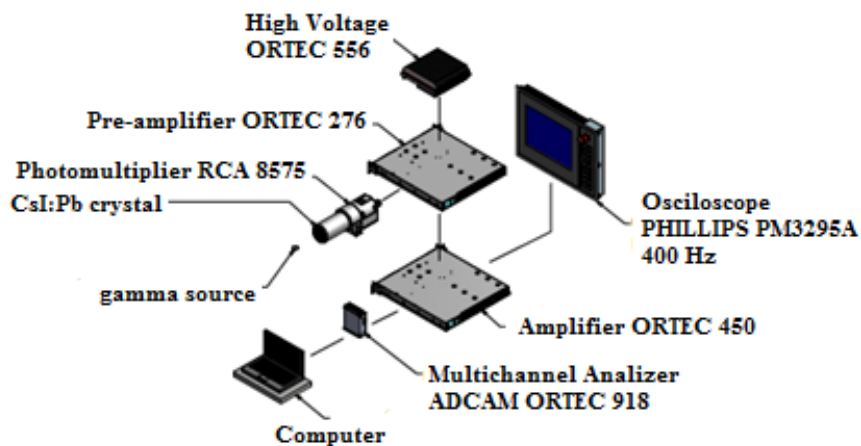
Figure 2: Schematic representation of the electronics associated with the CsI:Pb scintillator crystal coupled to the photomultiplier tube.
