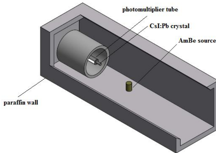
Figure 3: Exploded schematic representation of the array used for measurements.
