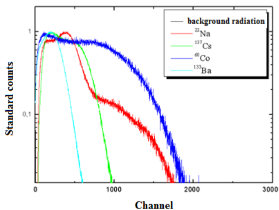
Figure 6: Spectra obtained for the radiation of ^{137}\text{Cs} , ^{60}\text{Co} , ^{22}\text{Na} e ^{133}\text{Ba} sources with CsI:Pb 5 \times 10^{-4} M crystal.
