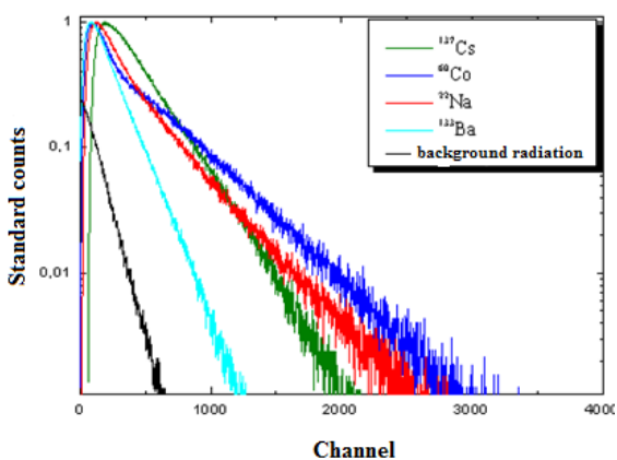
Figure 8: Spectra obtained for the radiation of ^{137}\text{Cs} , ^{60}\text{Co} , ^{22}\text{Na} e ^{133}\text{Ba} sources with CsI:Pb 1.5 \times 10^{-3} M crystal.
