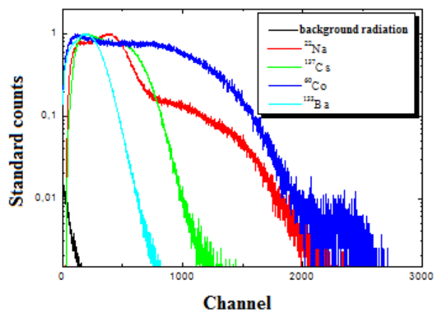
Figure 7: Spectra obtained for the radiation of ^{137}\text{Cs} , ^{60}\text{Co} , ^{22}\text{Na} e ^{133}\text{Ba} sources with CsI:Pb 10^{-3} M crystal.
