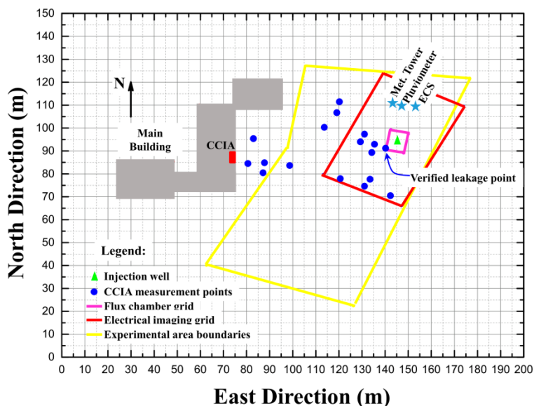
Figure 1: Schematic detail of the experimental cell and sampling locations.
