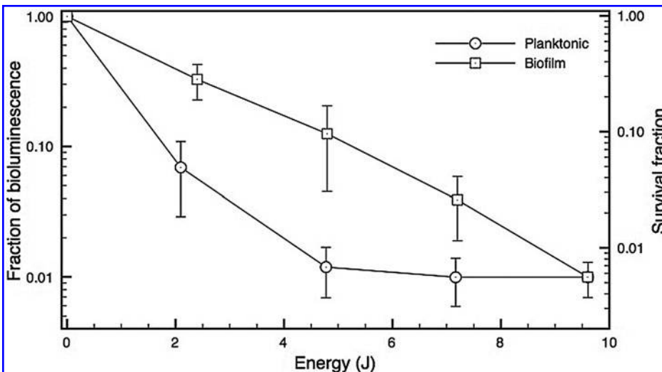
FIG. 3. Comparative loss of bacterial viability as measured by fraction of bioluminescence signal remaining after incubation with 60 μM methylene blue (MB) for 2 min and after photodynamic therapy (PDT) using 660-nm light on a Pseudomonas. aeruginosa suspension or intracanal biofilm.
