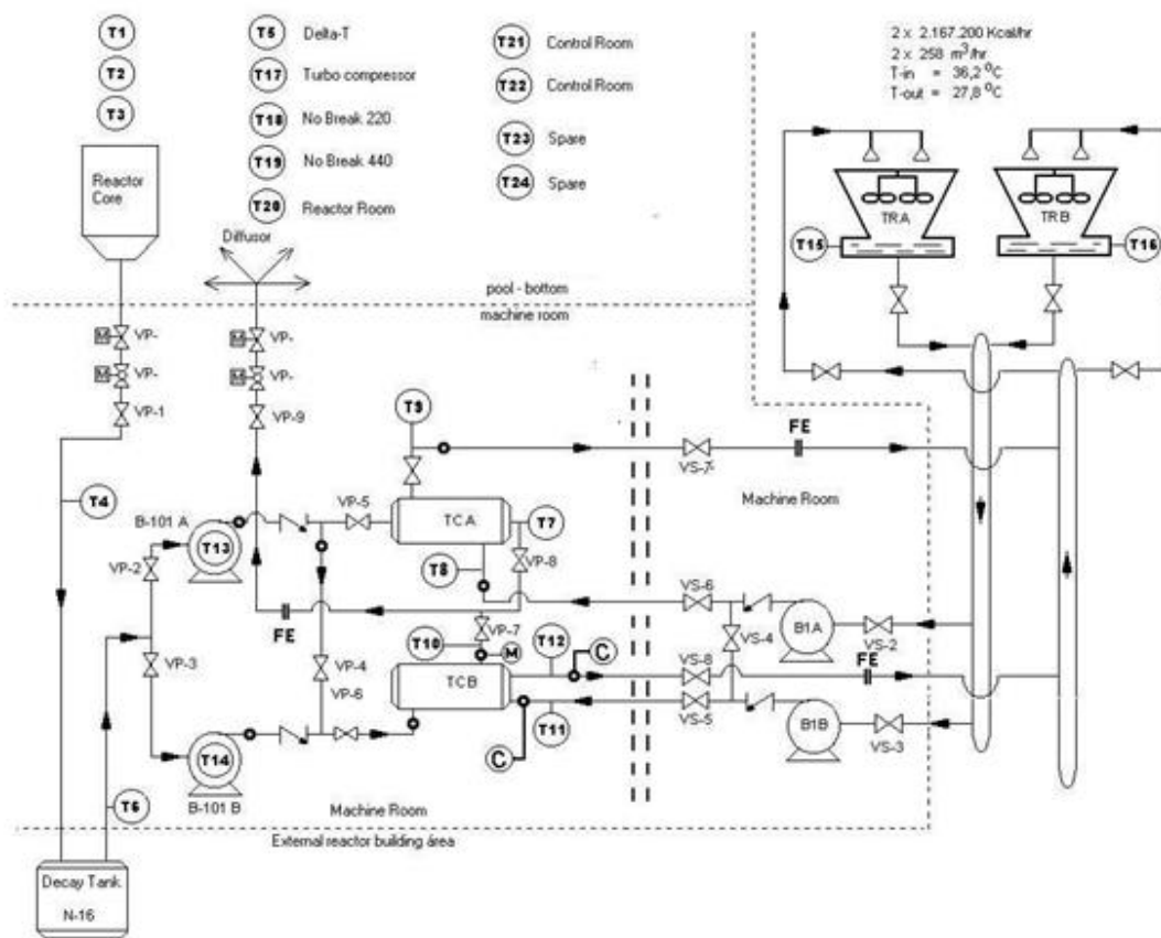
Figure 2. IEA-R1 experimental reactor schematic diagram
