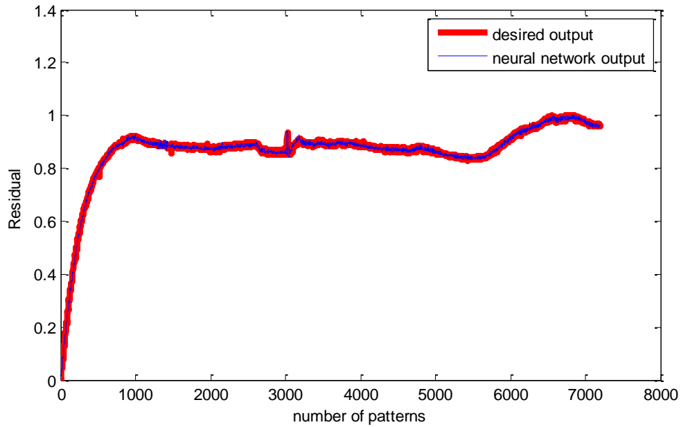
Figure 3: Neural network result for Temperature T3 monitoring.
