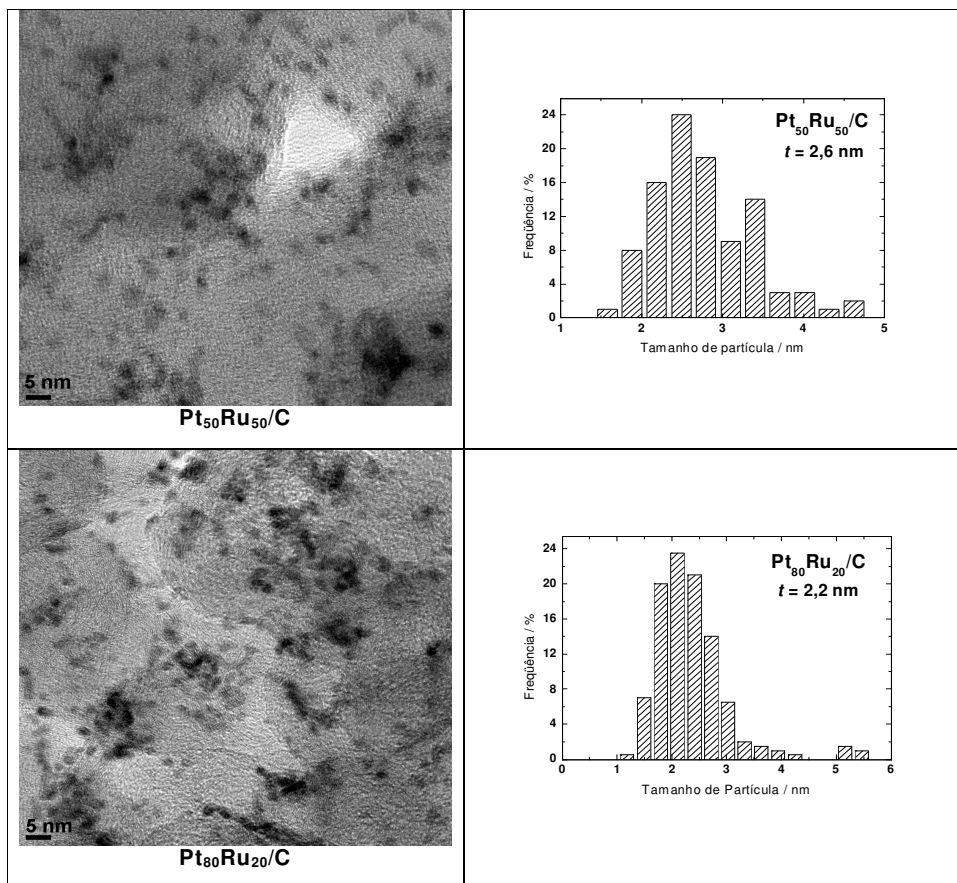
Figure 1. TEM micrographs and histograms of PtRu/C electrocatalysts
