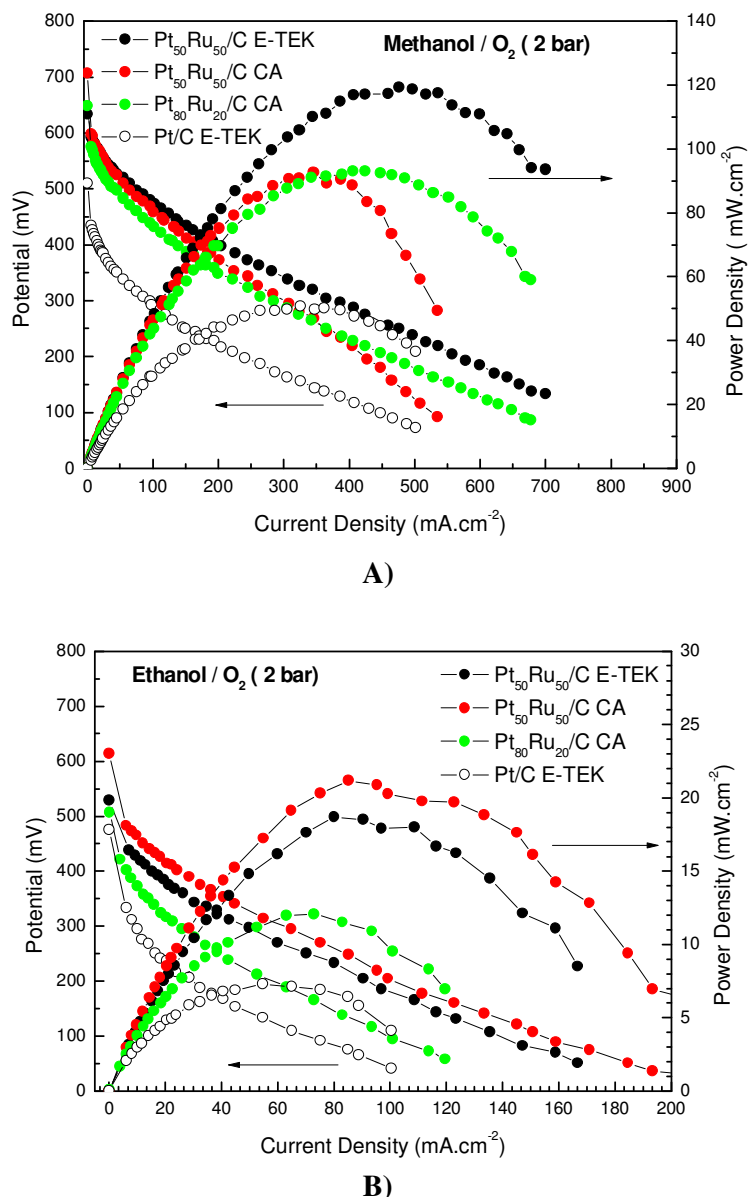
Figure 3. Electrical performances of a 5 cm² A) DMFC and B) at 90 °C using PtRu/C electrocatalysts (CA) and commercial Pt/C and PtRu/C (50:50) from E-TEK anodes (1 mg Pt cm⁻² catalyst loading) and Pt/C E-TEK cathode (1 mg Pt cm⁻² catalyst loading), Nafion 117 membrane, alcohol (2.0 mol L⁻¹), oxygen pressure (2 bar).
