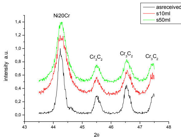
Fig. 2. X-ray diffraction patterns of the powders: AR (“as received”) and 50ml and 10ml of hexane are of powders milled for 8 hours.
