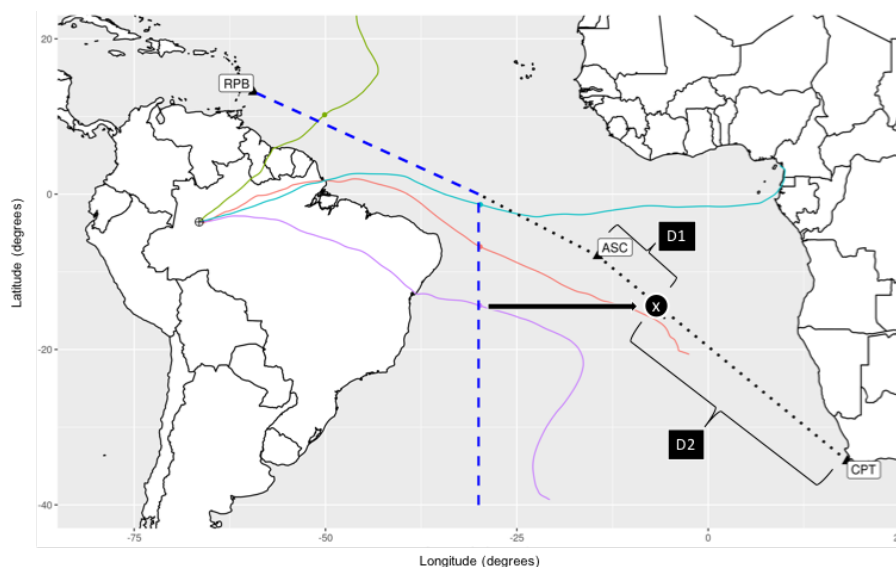
Figure 4. Air-mass back-trajectories method scheme. Blue dashed line is the Virtual Limit. Green, red, cyan and purple are examples of air-mass back-trajectories. D1 and D2 are the distances between the projected (black arrow) position “X” and the NOAA global stations, using the purple air-mass back-trajectory as an illustration of the AMBaM BKG calculation.
