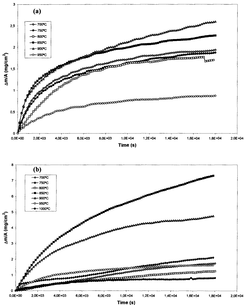
Fig. 13. Mass gain per unit area as a function of oxidation time for the composites (a) \text{Ni}_{20}\text{Cr}+5\%\text{WC} and (b) \text{Ni}_{20}\text{Cr}+10\%\text{WC} .
