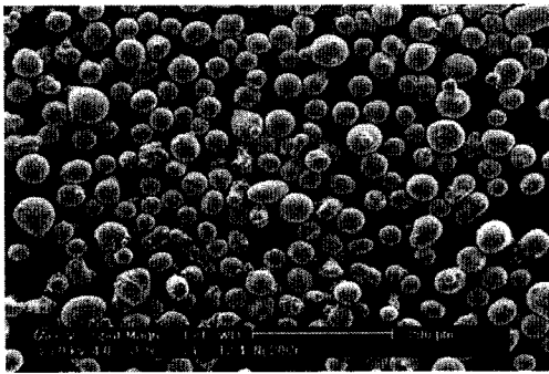
Fig. 1. Morphology of Ni20Cr powder.
