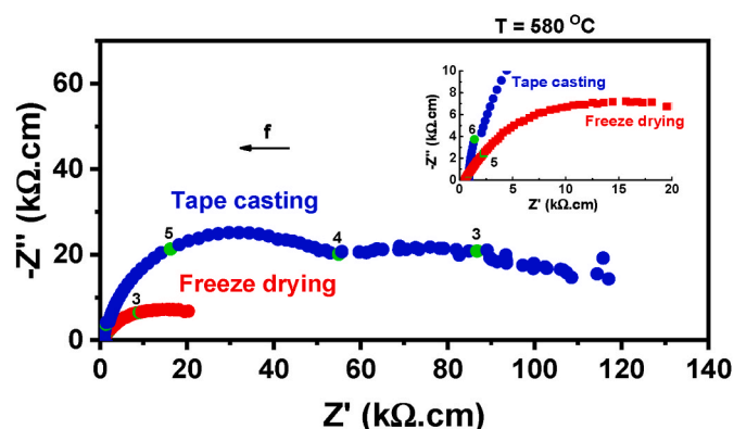
Fig. 6. Impedance spectroscopy diagrams of GDC porous samples produced by tape casting and freeze drying, sintered at 1450 °C. Temperature of measurement: 580 °C. Numbers stand for log f (f: Hz). Inset: zoom at the high frequency region.
