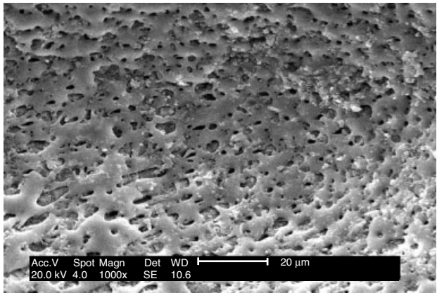
Figure 4 Dentin surface after CO 2 laser irradiation (9.6 μm, 150 mJ, 20 Hz, 212.2 J/cm 2 , 3 W); the melted surface partially occludes the dental tubules
