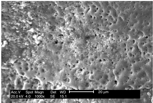
Figure 3 Enamel surface after CO 2 laser irradiation (9.6 μm, 150 mJ, 20 Hz, 212.2 J/cm 2 , 3 W); a melted surface is formed after the irradiation and the prismatic structure of the enamel is not seen
