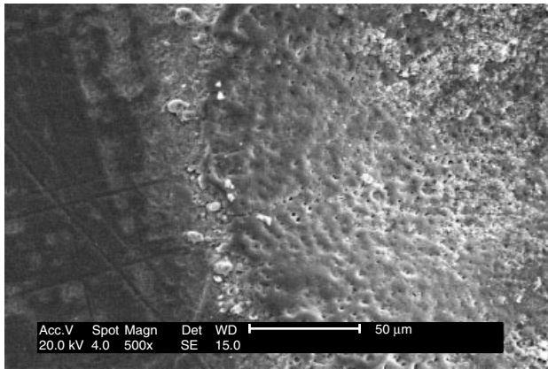
Figure 1 The natural enamel is observed in the left side of the figure and the CO 2 laser irradiated surface (9.6 μm, 150 mJ, 20 Hz, 212.2 J/cm 2 , 3 W) is observed in the right side
