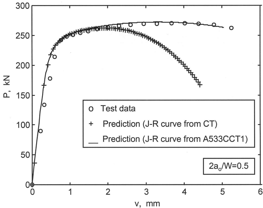
FIG. 6—Load versus displacement curve for A533CCT1
