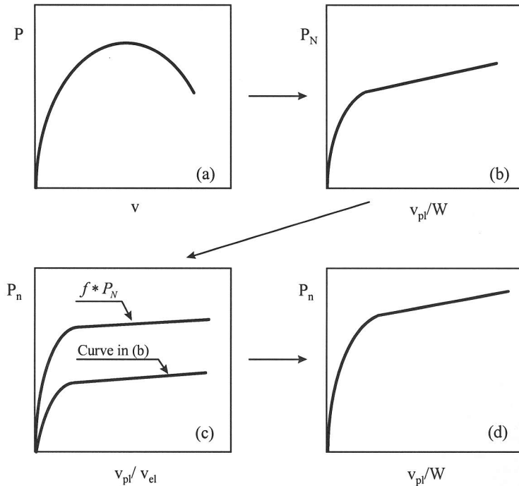
FIG. 2—Schematic of the original transformation procedure
