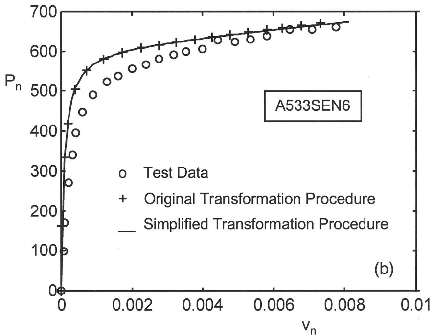
FIG. 4—Calibration curves for the SENS specimens
