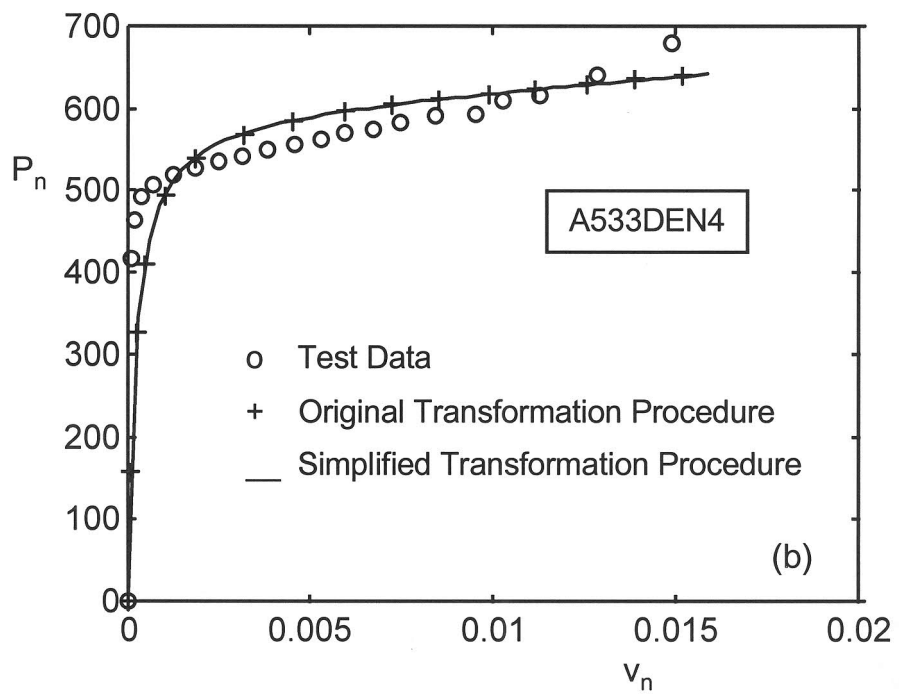
FIG. 5—Calibration curves for the DENT specimens
