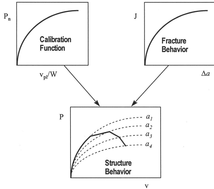
FIG. 1—Schematic of the Ductile Fracture Method
