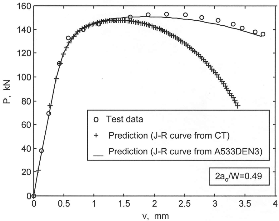
FIG. 8—Load versus displacement curve for A533DEN3
