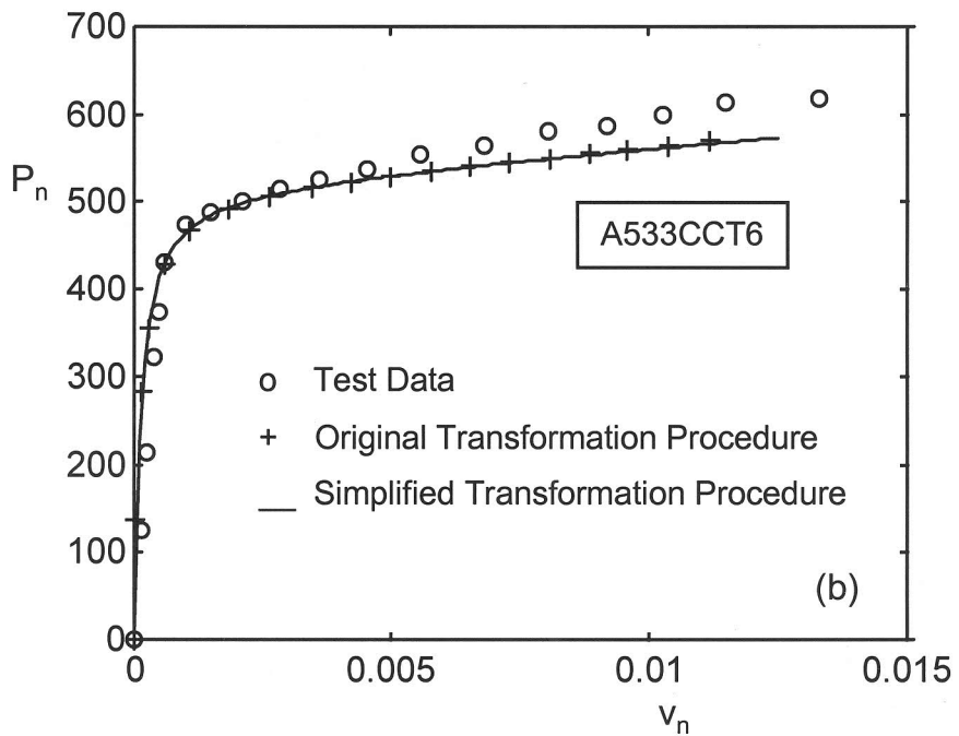
FIG. 3—Calibration curves for the CCT specimens
