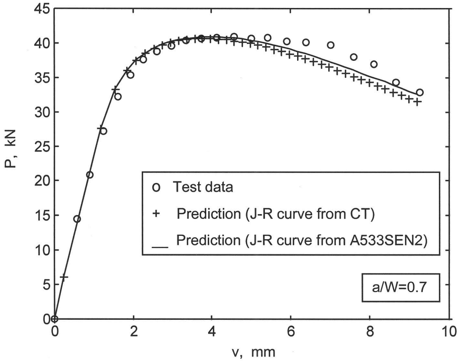
FIG. 7—Load versus displacement curve for A533SEN2
