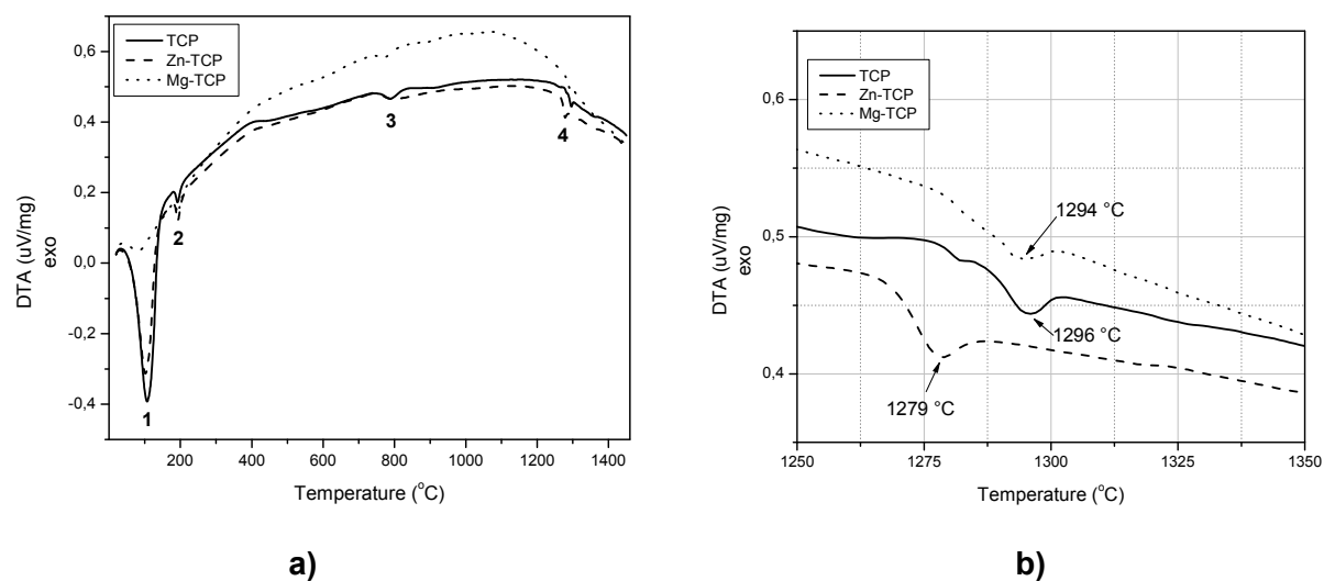
Fig 3: a) Differential thermal analysis results for TCP powder with different compositions. b) Enlarged region between 1250 – 1350°C, showing the detailed peak 4.
