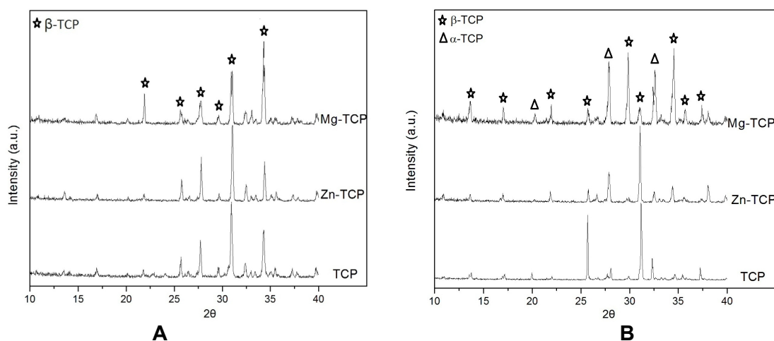
Fig. 5: XRD patterns of TCP samples sintered at different temperatures: (a): 1200°C/1h; (b): 1300°C/1h
