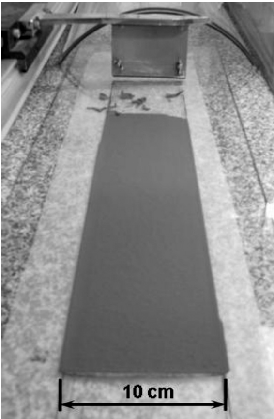
Fig. 6. As-cast tape of doped lanthanum chromite suspensions in ethanol with 55 wt% solids and 15 wt% BS.
