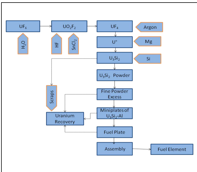
Fig. 1- Flowchart of fuel element manufacturing process of the CCN/IPEN [6]
