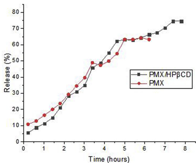
Fig. 8. In vitro release kinetics of free pramoxine (%) and the PMX/HP-β-CD complex (%), at pH 7 and 25 °C.
