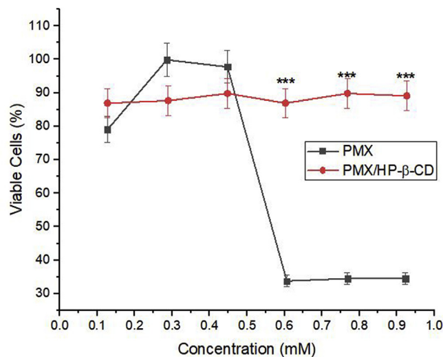
Fig. 9. Cell viability analysis (MTT test) of 3T3 fibroblasts (Balb/C) after treatment (24 h) with free (PMX) and complexed pramoxine (PMX/HP-β-CD). Data expressed as percentage of viable cells in relation to MTT control (mean \pm SD) n = 3 experiments. Statistical analysis: PMX vs PMX/HP-β-CD. Unpaired T test: *** p < 0.001 .
