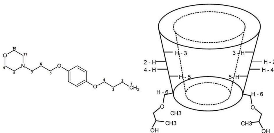
Fig. 1. Chemical structure of pramoxine and hydroxypropyl beta-cyclodextrin (HP-β-CD). Numbers refer to ^1\text{H} NMR peak assignment.
