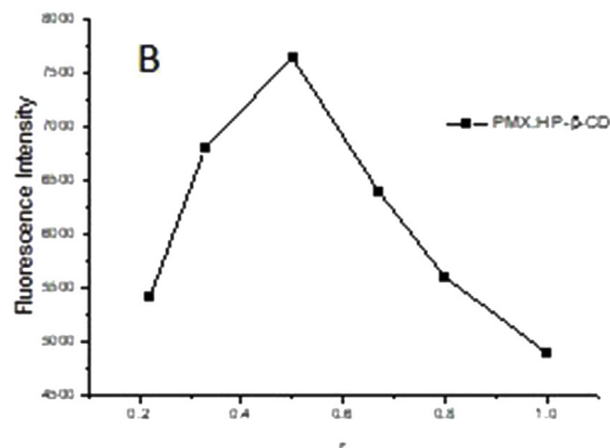
Fig. 3. A) Fluorescence emission spectra of PMX (0.06 mM) complexed with HP-β-CD, at different PMX/HP-β-CD molar ratios ( r ), at pH 7.4 and room temperature. B) Continuous variation (Job Plot), showing changes in the anesthetic fluorescence as a function of r , used to determine the PMX/HP-β-CD complex stoichiometry.
