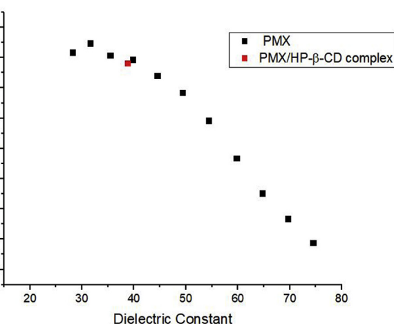
Fig. 4. Intrinsic fluorescence of PMX (1 mM) at increasing dielectric constant, and in the PMX/HP-β-CD complex, at pH 7.4.
