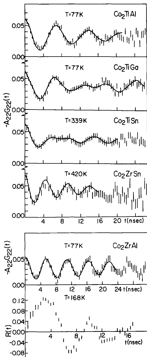
Fig. 1 - TDPAC results for ^{181}\text{Ta} at the Y site of Heusler alloys \text{Co}_2\text{YZ} ( Y = \text{Ti, Zr} ; Z = \text{Al, Ga, Sn} )
