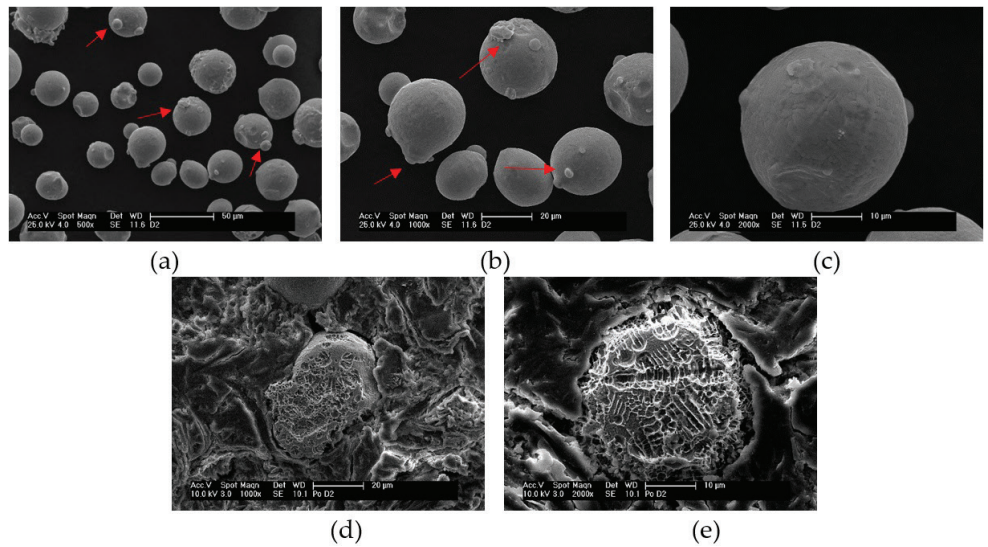
Figure 7. SEM images of Co-Cr-Mo powder: (a) magnitude ×500, (b) magnitude ×1000, (c) magnitude ×2000, (d) and (e) cross-section powder after chemical etch (etch solution: HCl, H 2 SO 4 , and HNO 3 for 60–240 s at 45°C, respectively, magnitude ×1000 and ×2000).
