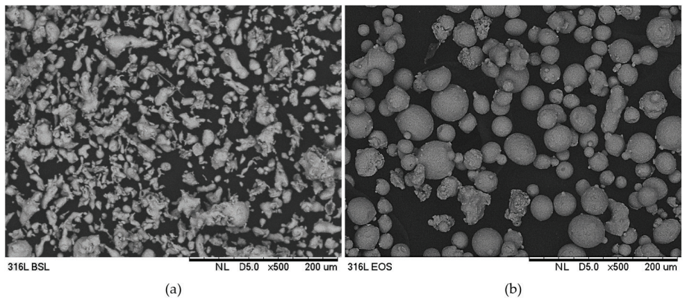
Figure 5. Characteristic format of powders (316L alloy) produced by water atomization (a) and gas atomization (b). Magnitude x500.
