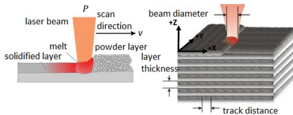
Figure 3. Schematic of parameters involved in SLM consolidation [31].
