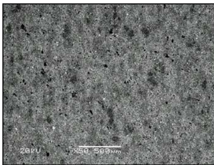
Figure 3. SEM micrograph of alloy 2 in the as sintered condition.
