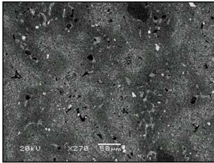
Figure 8. SEM micrograph of alloy 2 in the as sintered condition.
