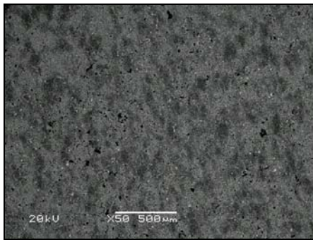
Figure 1. SEM micrograph of alloy 1 in the as sintered condition.
