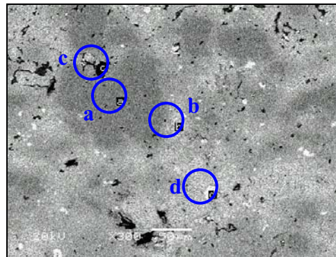
Figure 10. SEM micrograph of alloy 2 in the as heat-treated condition.
