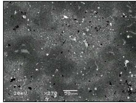
Figure 9. SEM micrograph of alloy 2 in the as sintered and heat treated condition.
