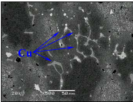
Figure 5. SEM micrograph of alloy 1 in the as sintered condition.
