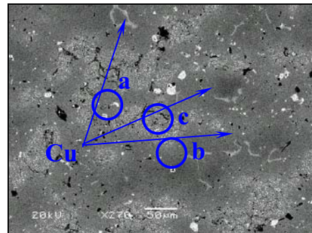
Figure 6. SEM micrograph of alloy 1 in the as sintered and heat treated condition.
