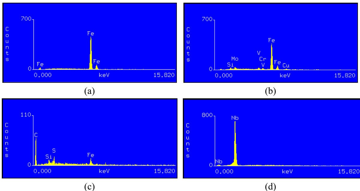
Figure 11 – Spectra obtained by EDS, of the areas a, b, c and d, of Fig. 10.
