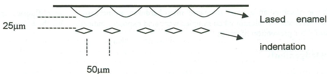
Figure 01 - Conditions of hardness measurements
