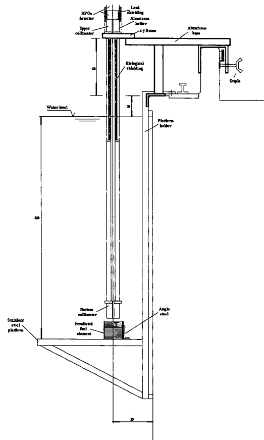
Figure 4. Cross-sectional diagram of the experimental apparatus for gamma-ray spectroscopy installed at the pool area of the IEA-R1 research reactor. Dimensions are in cm.
