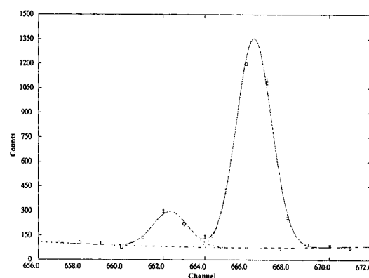
Figure 7. Gaussian functions fitted to each full-energy peak of the doublet with energies 657.7 keV ( ^{110\text{m}}\text{Ag} ) and 661.6 keV ( ^{137}\text{Cs} ) using the computer program IDEFIX [18], in order to separate the areas of these peaks in the gamma-ray spectrum obtained from measurement at the central point of the fuel element 111.
