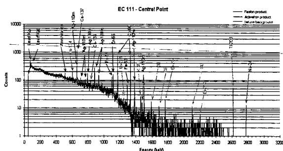
Figure 6. Gamma-ray spectrum obtained from measurements of 600 s of live time performed at the central point of the irradiated fuel element 111. The origin of each peak is indicated.
