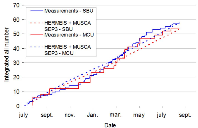
Fig. 9. Measured and calculated SEU events including the SBU and MCU events (MUSCA SEP 3 using the HERMEIS spectra as inputs).
