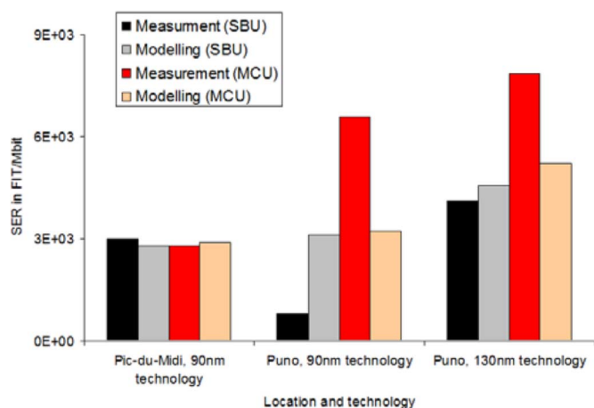
Fig. 13. Comparison between the measured and calculated SER (distinguishing the SBU and MCU events) for the 90- and the 130-nm devices and for both high-altitude locations (Pic-du-Midi and Puno).
