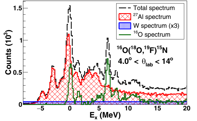
FIG. 4. Decomposition of the excitation energy spectrum obtained with the \text{WO}_3 + ^{27}\text{Al} target. The total spectrum is presented with the dashed black line. The red-hatched area corresponds to the normalized background originating from the ^{27}\text{Al} backing material, while the dotted blue area corresponds to the background arising from the tungsten component of the target. For reasons of clarity, the latter is multiplied by a factor of 3. The histogram illustrated by the solid green line is the obtained excitation energy spectrum for the ^{16}\text{O}(^{18}\text{O}, ^{19}\text{F})^{15}\text{N} reaction, after subtracting from the total spectrum the background contributions.
