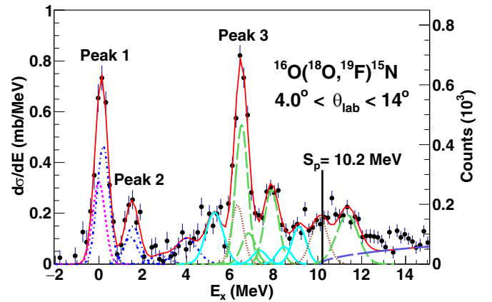
FIG. 5. Excitation energy spectrum for the ^{16}\text{O}(^{18}\text{O}, ^{19}\text{F})^{15}\text{N} reaction at the energy of 275 MeV compared to the results of the fit procedure, where for the description of each state a Gaussian function was used. The adopted colors and line styles are the same as those presented in Fig. 2. In addition to Fig. 2, in the case of several nearby states a single Gaussian function, depicted with the double-dotted-dashed curve, was considered in the fit procedure with the centroid fixed to the mean value of the excited states. Moreover, the continuum background above the proton emission threshold of ^{15}\text{N} is indicated with the purple line.
