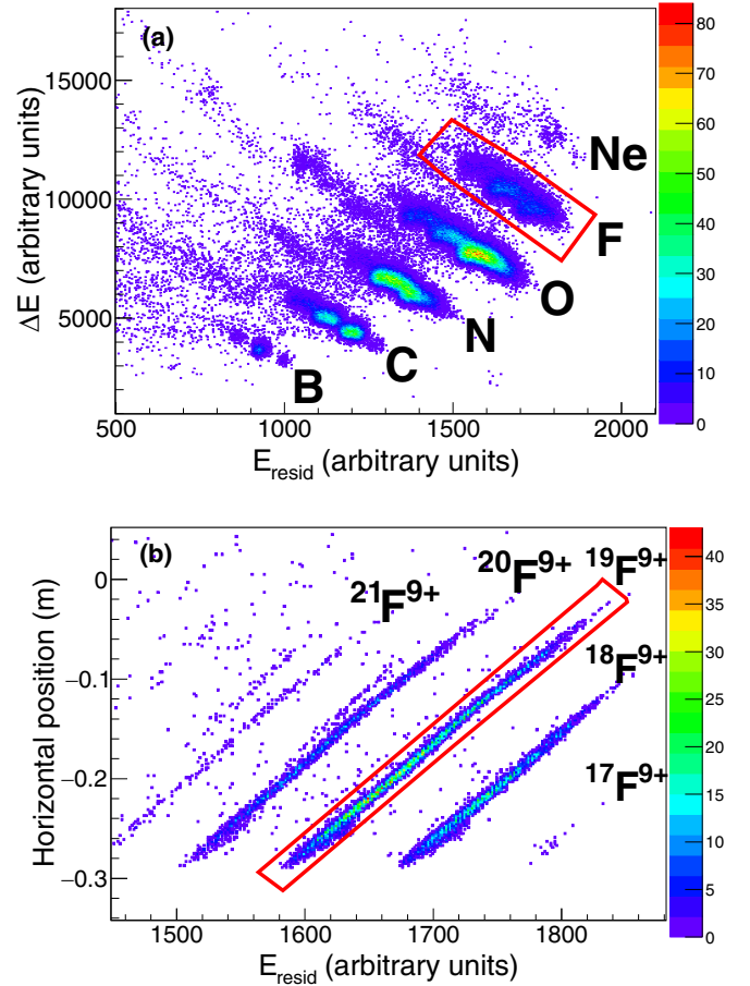
FIG. 1. Typical identification spectra for ^{48}\text{Ti}(^{18}\text{O}, ^{19}\text{F})^{47}\text{Sc} reaction at the energy of 275 MeV. (a) \Delta E - E_{\text{resid}} correlation plot for the ions energy loss inside the gas tracker, \Delta E , as a function of the residual energy, E_{\text{resid}} , measured by one silicon detector of the FPD. A graphical selection in the contour of the fluorine ion events is illustrated by the solid red line. (b) The horizontal position at the MAGNEX focal plane as a function of the residual energy for the selected fluorine ions of panel (a). The different loci correspond to ions with different ratio \sqrt{m}/q . A graphical selection on the ^{19}\text{F}^{9+} events is shown by the solid red line.
