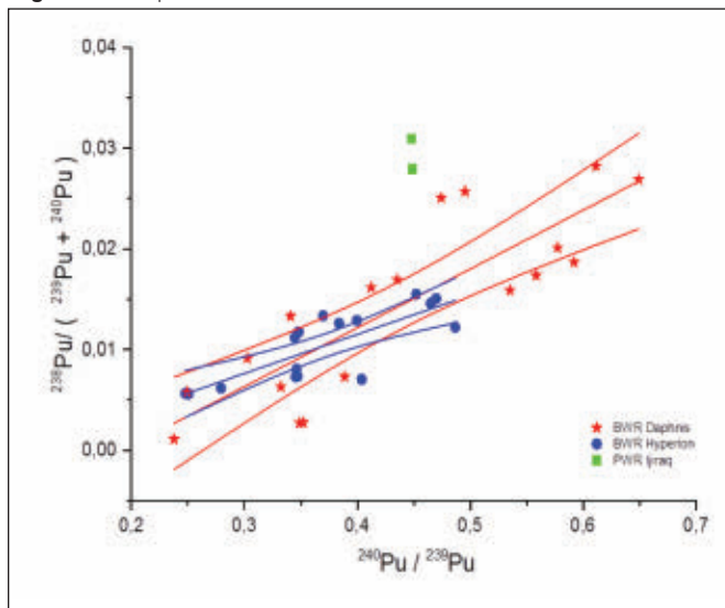
Figure 2. Isotopic Correlation: ^{238}\text{Pu}/(^{239}\text{Pu}+^{240}\text{Pu}) versus ^{240}\text{Pu}/^{239}\text{Pu}
