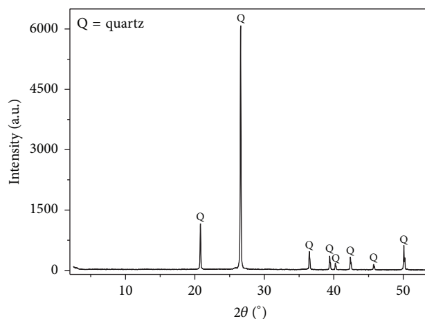
FIGURE 2: X-ray diffractogram of sugarcane biomass ash.
