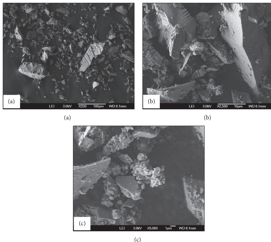
FIGURE 6: Scanning electron microscopy of biosilica. Magnification of 250x (a), 2500x (b), and 5000x (c).
