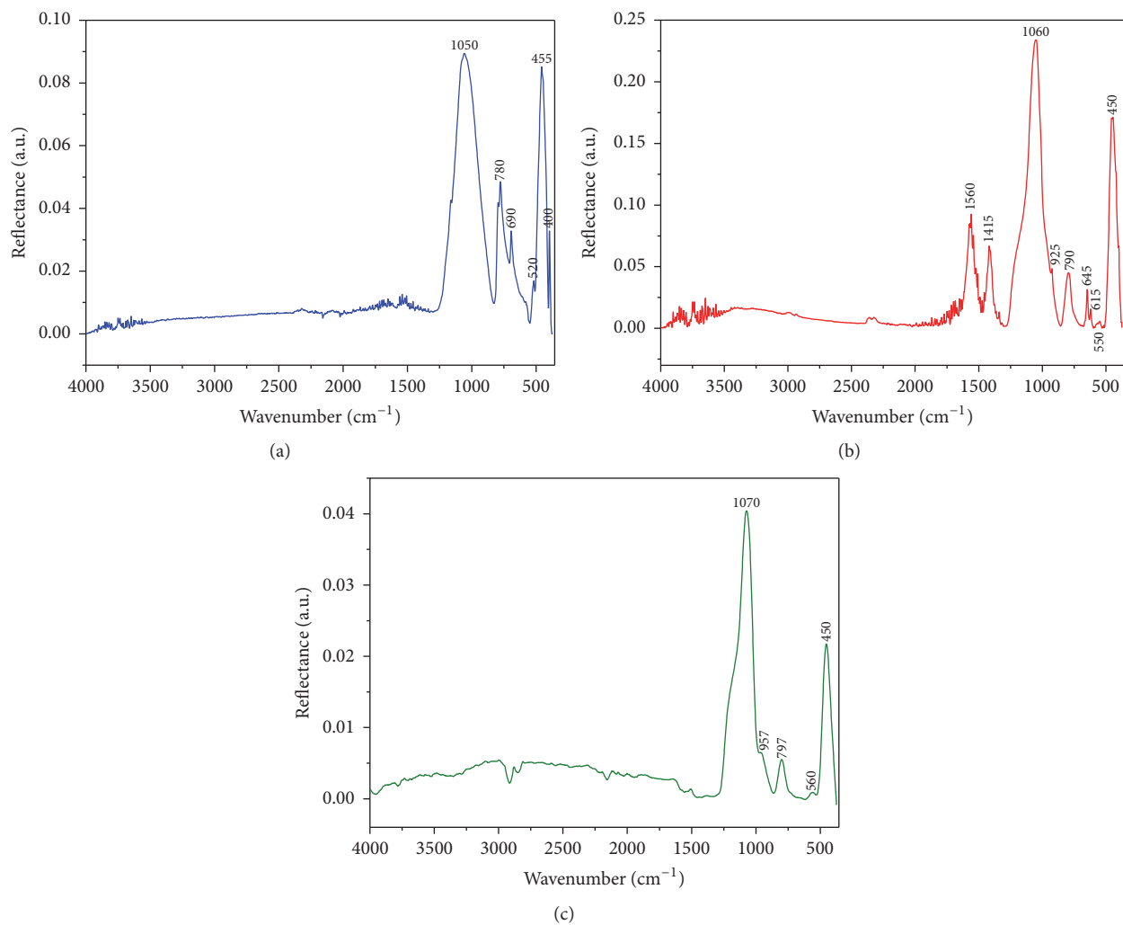
FIGURE 8: FTIR vibrational spectra for the samples: sugarcane waste ash (a), biosilica (b), and biosilica washed with water (c).
