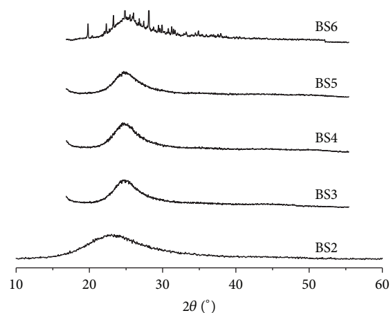
FIGURE 4: XRD patterns of the synthesis products obtained by hydrothermal treatment of sugarcane waste ash at 100°C.
