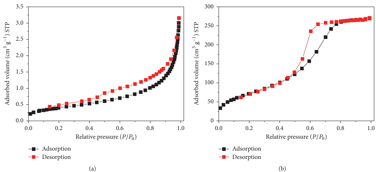
FIGURE 9: Nitrogen adsorption-desorption isotherms for the samples: ash (a) and biosilica (b).
