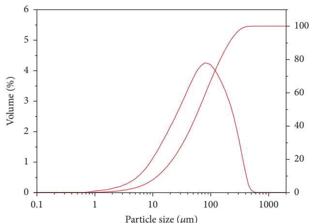
FIGURE 3: Particle size distribution curves of sugarcane biomass ash.
