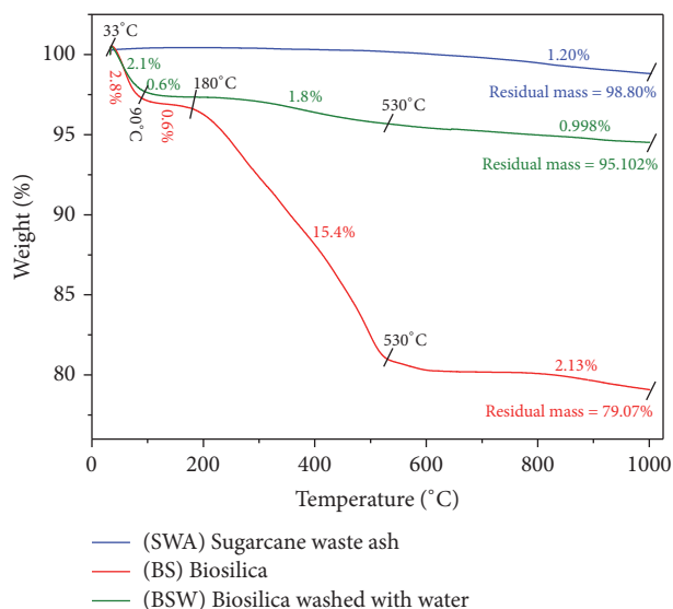
FIGURE 7: TG curves of SWA (blue), BS (red), and BSW (green) under an inert atmosphere of nitrogen.
