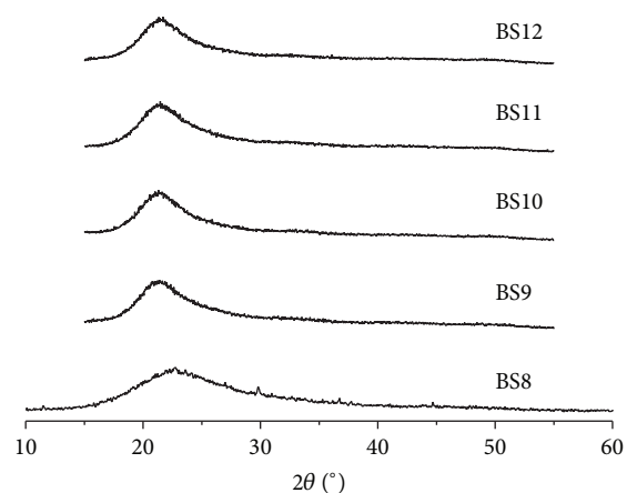
FIGURE 5: XRD patterns of the synthesis products obtained by hydrothermal treatment of sugarcane waste ash at 90°C.
