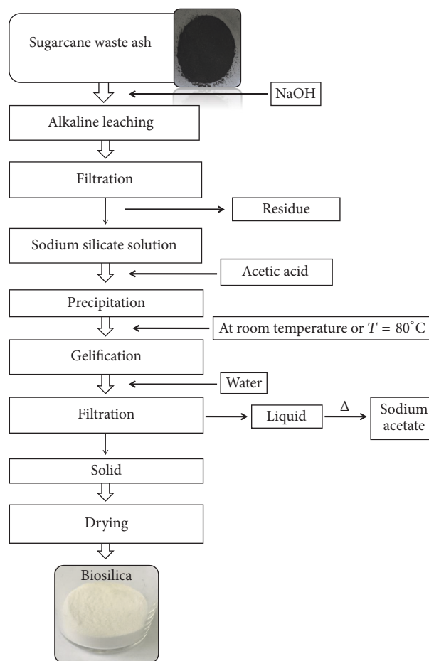
FIGURE 1: Flow diagram of the procedure used to produce biosilica from sugarcane biomass ash.
