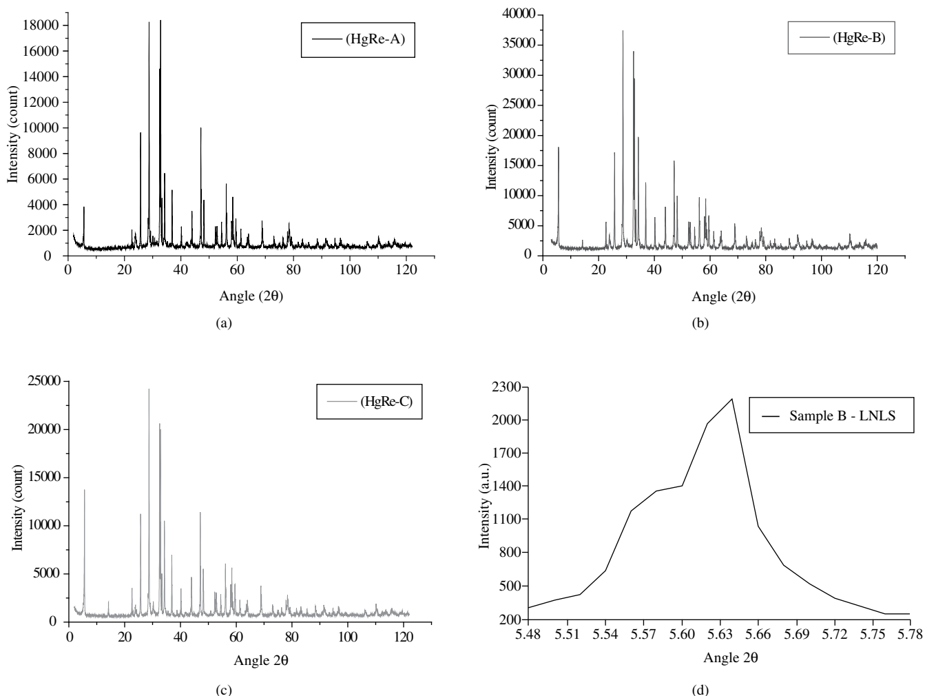
Figure 2. XRD for the samples a) A, b) B and c) C with \text{Cu}_{k-\alpha} radiation and d) detail of the 001 reflection using high resolution Synchrotron diffraction.
