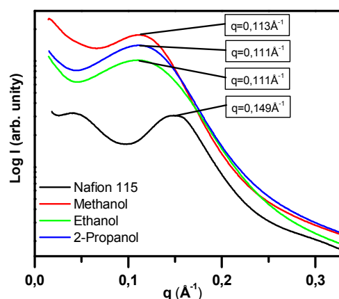
FIGURE 2: Small-angle X-ray scattering in wet state for Nafion and Nafion-SiO 2 hybrids synthesized in different environments
