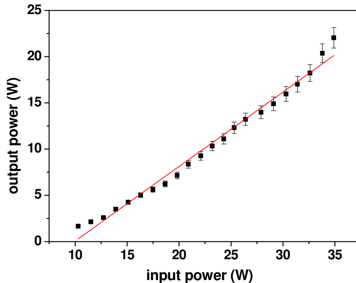
Fig. 2: Output power versus diode pump power.
