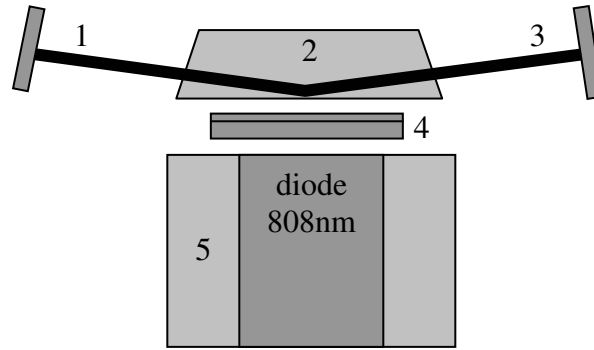
Fig. 1 Cavity configuration: 1) end mirror ( R=50 cm); 2) a-cut \text{Nd:YVO}_4 crystal; 3) plane output mirror with 36% transmission; 4) 6.4 mm cylindrical lens; 5) 20 W, TM-polarized diode bar.
