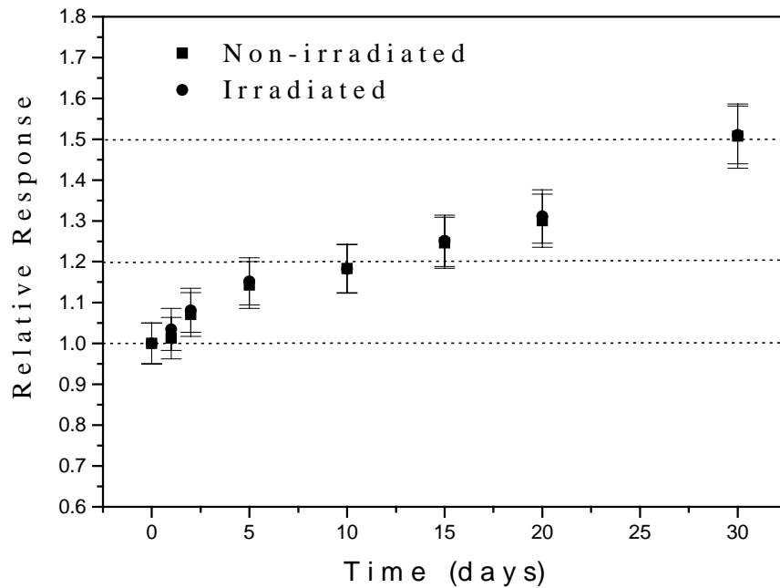
FIG. 5. Relative response obtained with solutions obtained using pellets (40% MnO_2 / 60% KNO_3 ) irradiated with 200kGy, prepared and evaluated after up to 30 days of storage.
