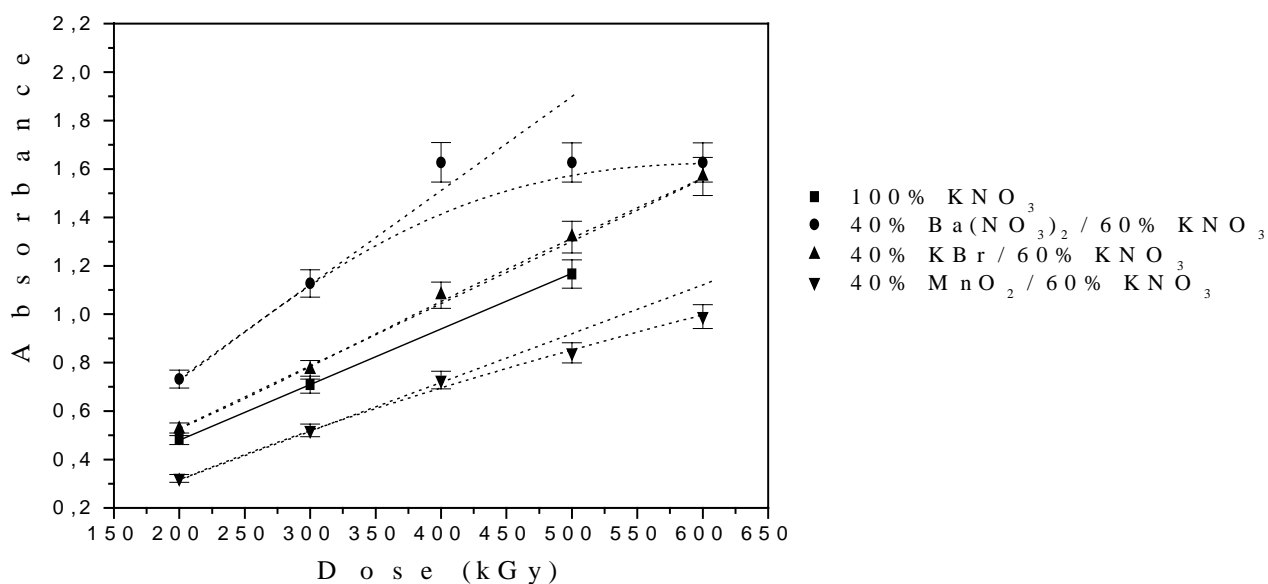
FIG. 6. Dose-response curves of pellets of \text{KNO}_3 p.a and pellets of mixtures with \text{Ba}(\text{NO}_3)_2 , \text{KBr} and \text{MnO}_2 , irradiated with gamma dose between 200 kGy and 600 kGy.
