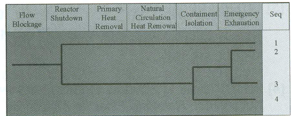
Figure 1. Event Tree for Flow Blockage
