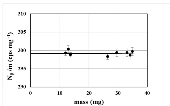
Figure 2. Self-absorption extrapolation curve of ^{32}\text{P} 4\pi(\text{PC})\text{-}\beta system. The black marks correspond to experimental points and the continuous line to the fitting.
