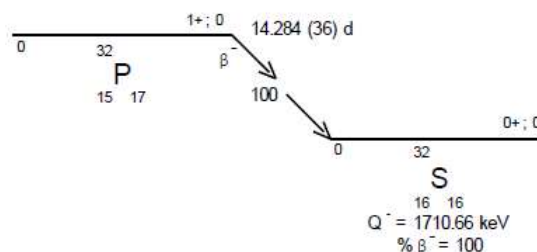
Figure 1. ^{32}\text{P} decay scheme [Christé, 2004]
