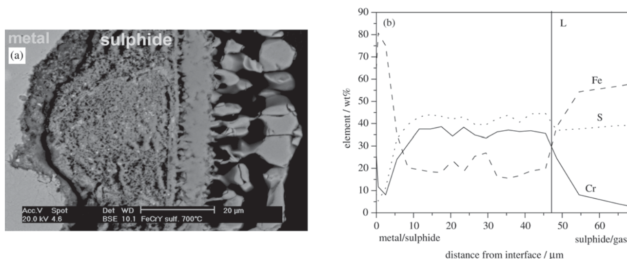
Figure 4. a) cross-section of FeCrY alloy sulphidised at 700 °C; b) composition profile through a).
