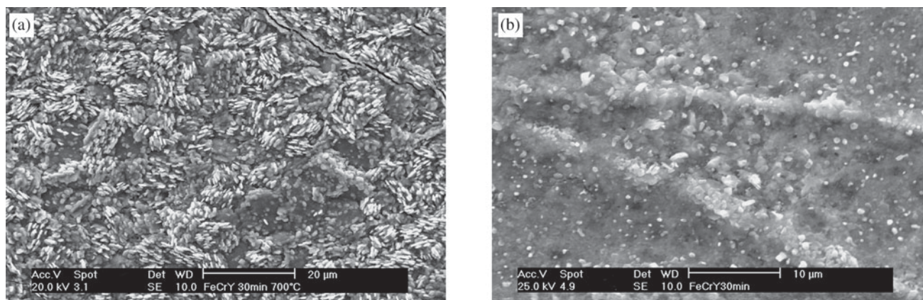
Figure 10. Surface of the FeCrY alloy sulfidized for 30 min at 700 °C.
