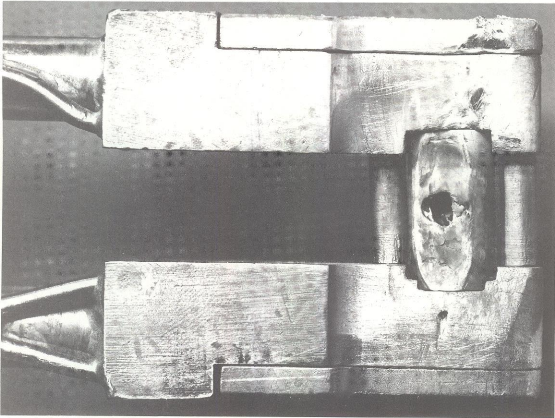
Figure 2: Worn out ion source.
