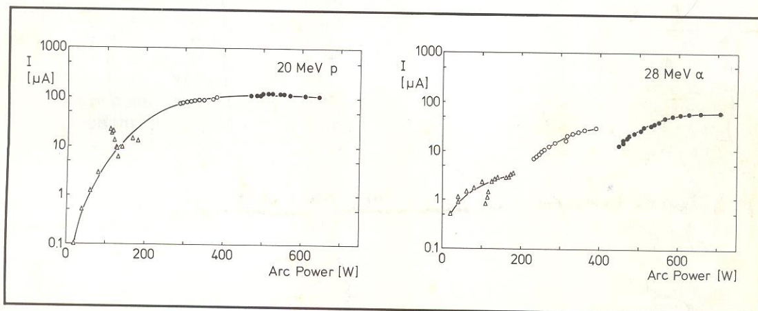
Figure 5a: Dependence of the ion beam current on the arc power; \Delta : PIG mode; \circ : low thermionic mode; \bullet : high thermionic mode.
