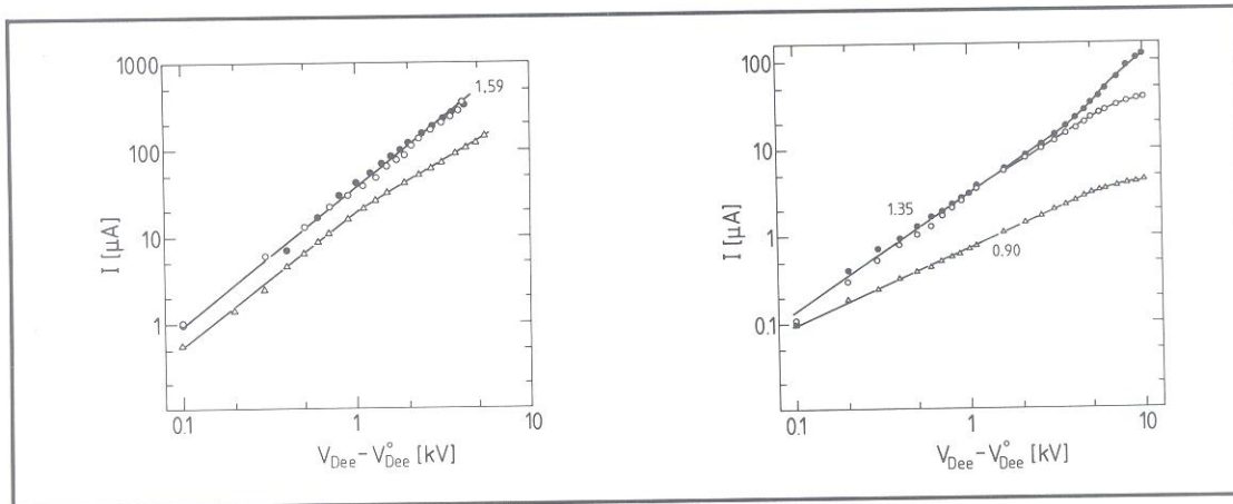
Figure 3b: Dependence of \alpha -beam current at 0.15 \text{ m} radius on Dee-Voltage for different modes of operation in a log-log plot \Delta : PIG mode; \circ : LT mode; \bullet : HT mode.
