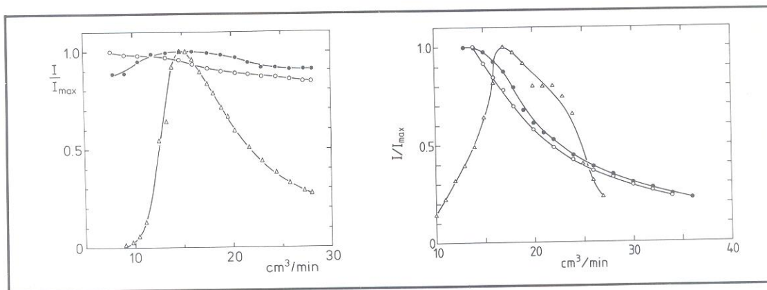
Figure 4b: Dependence of normalized beam current at 0.15 \text{ m} radius for 28 \text{ MeV} \alpha on He flow rate. \Delta : PIG, I_{\text{max}} = 3.5 \mu\text{A} ; \circ : LT mode, I_{\text{max}} = 29.5 \mu\text{A} ; \bullet : HT mode, I_{\text{max}} = 60.5 \mu\text{A} .
