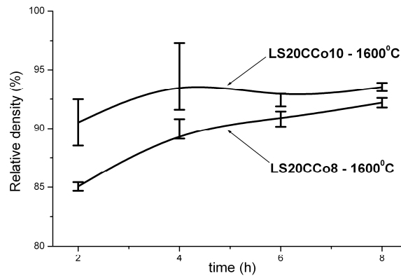
Figure 4 - Sintered densities data for compositions LS20CCo8 and LS20CCo10 after sintering at 1600°C.
