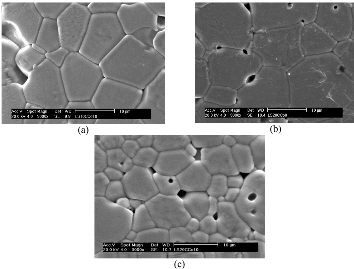
Figure 5 – Micrographs (MEV) from the compositions (a) LS10CCo10, (b) LS20CCo8 and (c) LS20CCo10.
