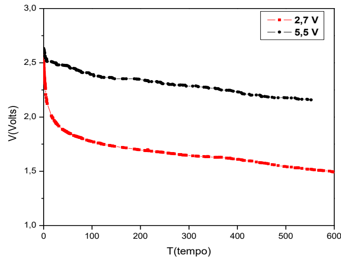
Figure 4. Self-discharge curves for the carbon based supercapacitors at room temperature.
